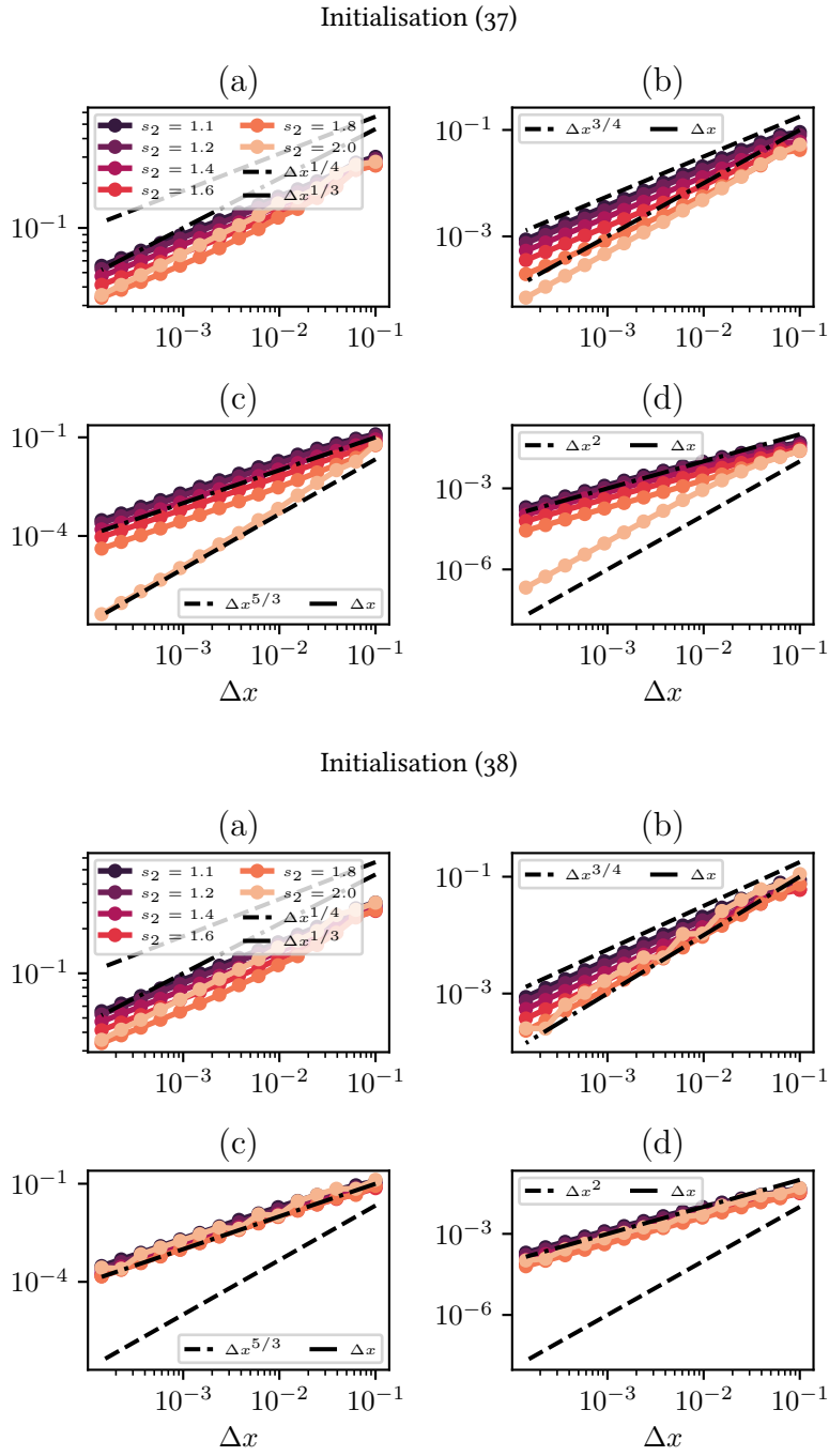
Figure 3: L^2 errors at the final time for two forward centered initialisations (37) (top) and (38) (bottom). Since the letter irredeemably perturbs the conserved moment feeding the bulk Finite Difference scheme, the orders of convergence above one are lowered.
