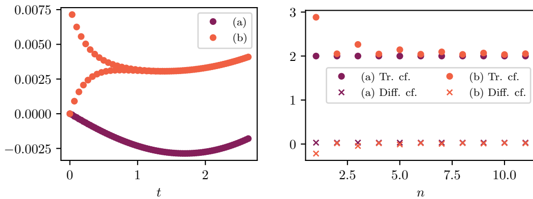
Figure 11: Left: test for smoothness in time close to t = 0 for for the initialisations (a) and (b): difference between exact and numerical solution at the eighth lattice point. The first one gives a smooth profile whereas the second one oscillates with damping. Right: transport and diffusion coefficient in the modified equations for different n .
