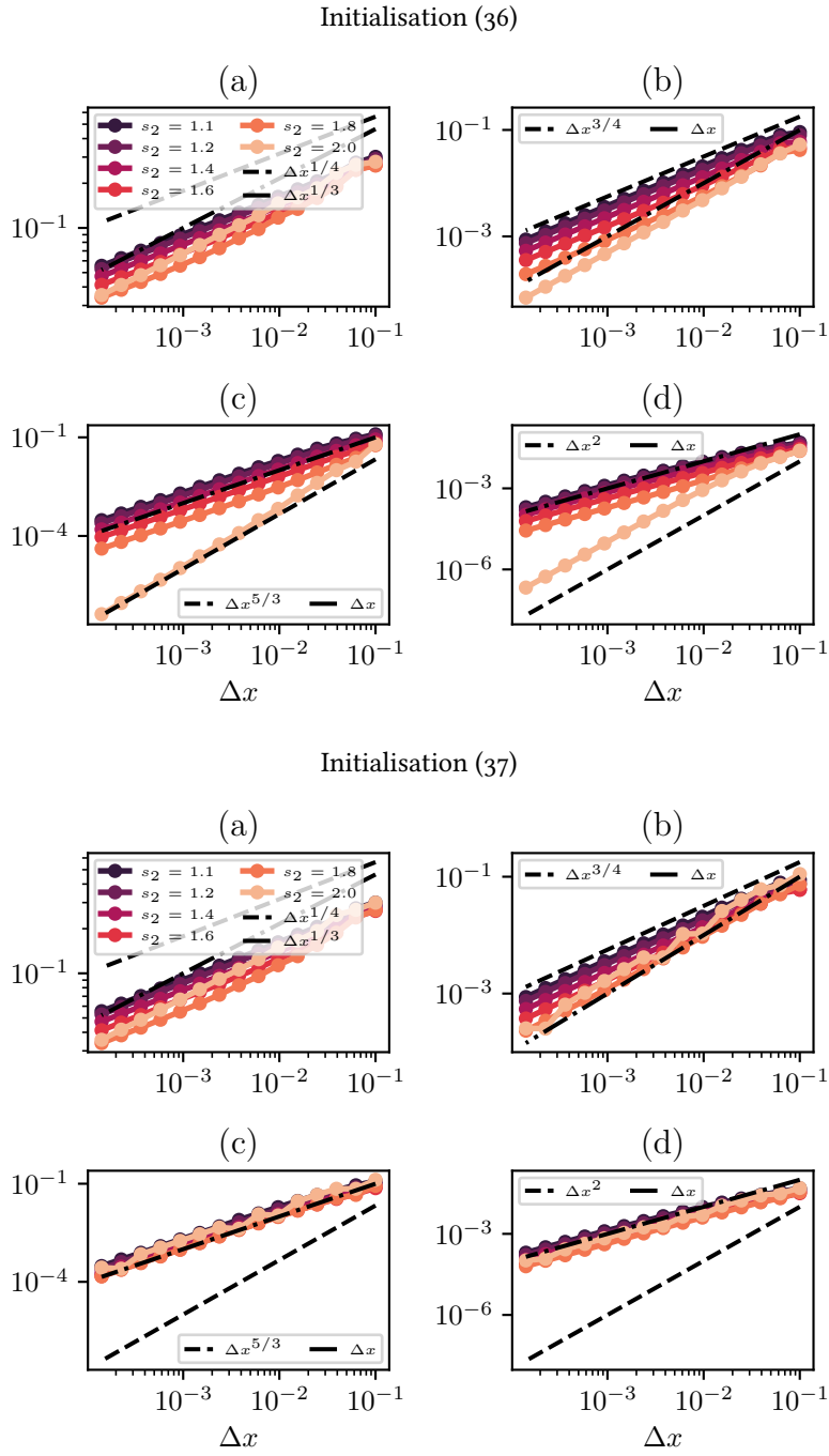
Figure 3: L^2 errors at the final time for two forward centered initialisations (36) (top) and (37) (bottom). Since the letter irredeemably perturbs the conserved moment feeding the bulk Finite Difference scheme, the orders of convergence above one are lowered.
