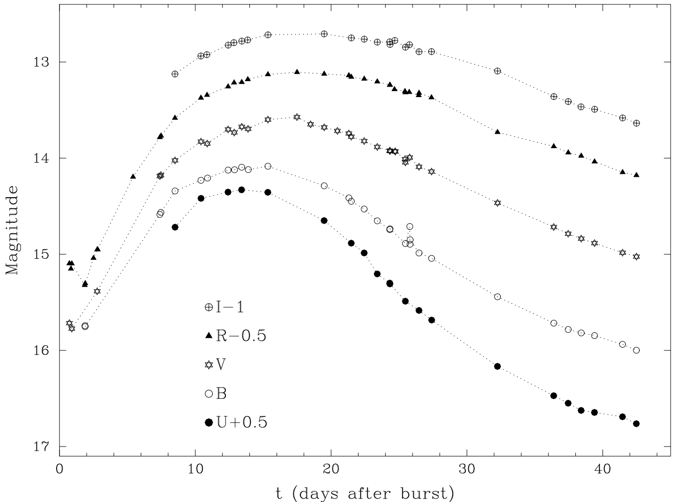
SN 1998 bw light curves
