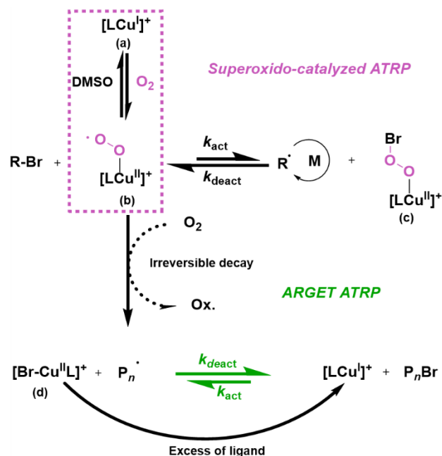
Scheme 1: Proposed mechanism of ligand of oxygen-enhanced ATRP.
