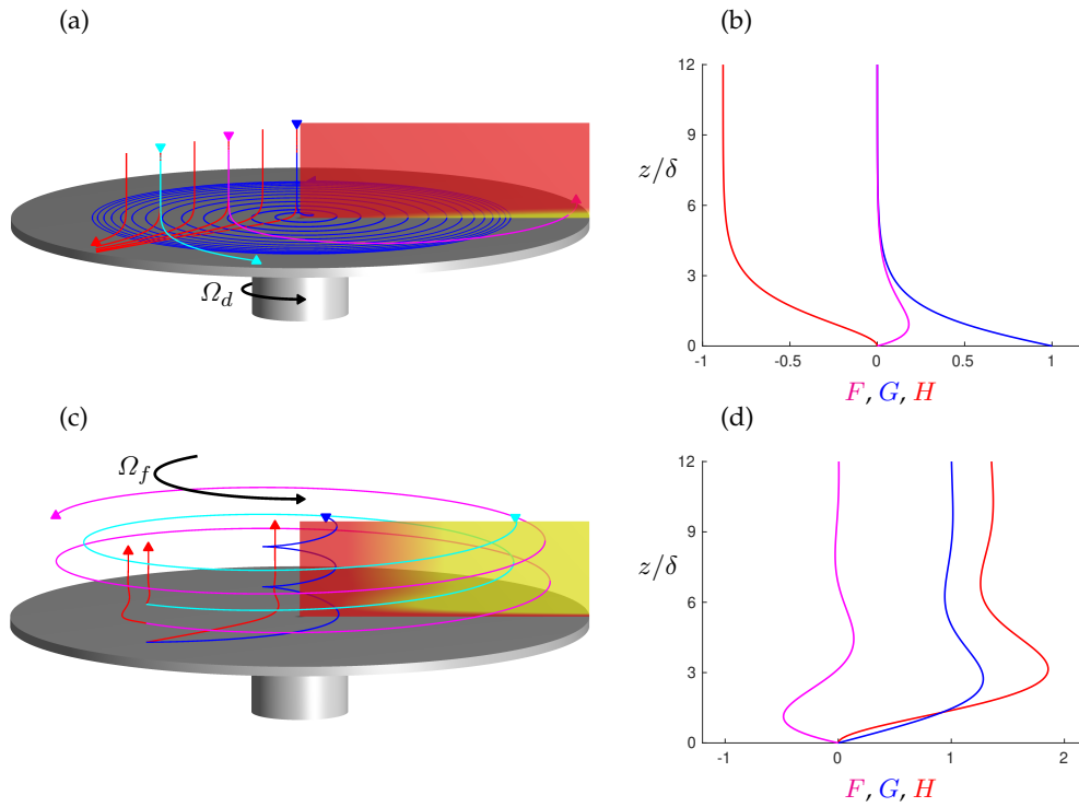
Figure 1: Similarity solutions in a single disk configuration. (a) and (b): Von Kármán solution over a rotating disk and (c) and (d): Bödewadt solution over a stationary disk, both in the inertial frame. The meridional planforms in (a) and (c) show the azimuthal component of the velocity. A few streamlines in the whole space are depicted by the blue, magenta and cyan curves and the corresponding streamlines restricted to a meridional plan by red ones. (b) and (d): Axial shape functions F (magenta), G (blue) and H (red) of the velocity profile, as functions of z/\delta .
