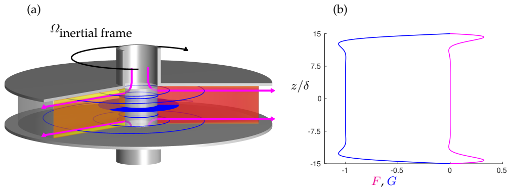
Figure 3: Rotating open cavity flow in the rotating frame of reference. (a) The meridional plan on the right shows the azimuthal component of the velocity and the one on the left the radial component. A few streamlines are depicted in blue and the imposed radial flux in magenta. (b) Axial shape functions F (magenta) and G (blue) of the velocity profile, as functions of z/\delta .
