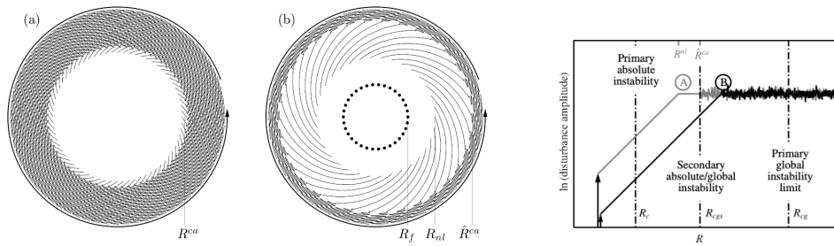
Figure 7: Sketches showing the two classes of transition scenario in the single-disk configuration: (a) The absolute scenario: onset of a primary absolute instability characterized by a steep front and spiral arms immediately followed downstream by secondary absolute instability and turbulence. (b) The convective scenario: onset of a primary convective instability excited by self-sustained perturbations, nonlinear saturation and secondary absolute instability downstream leading to turbulence. (c) In the convective scenario, transition to turbulence for disturbances with two different amplitudes. (a, b) a copy of Figure 3 of Ref. [67]. (c) A copy of Figure of Ref. [63]. R^{ca} , R_f , R^{nl} , and \hat{R}^{ca} denote respectively the critical Reynolds numbers of the local absolute primary instability, of the forcing, of the nonlinear saturation of the primary convective instability and of the absolute global secondary instability.
