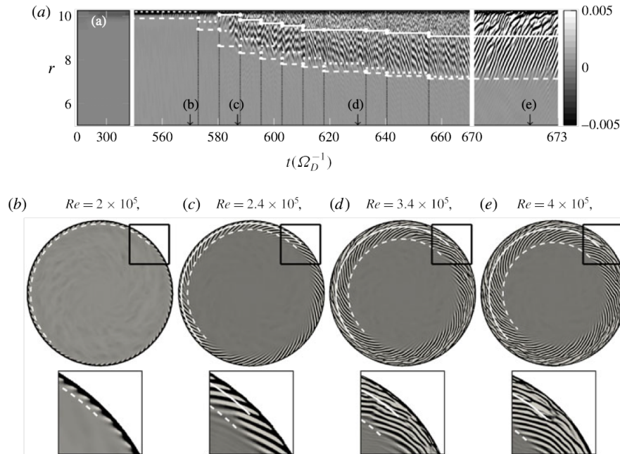
Figure 10: Temporal evolution of the flow patterns in the rotor boundary layer of the cylindrical rotor-stator cavity when increasing Reynolds number in the range Re \in [2 \times 10^5, 4 \times 10^5] , a copy of Figure 4 of Ref. [44]. (a) Spatio-temporal diagram. (b–e) Instantaneous top views of axial velocity field w corresponding to four Re , at time instants as indicated on (a). The white dashed (– –) and solid (—) lines in (a–e) show the positions of the primary and secondary fronts, respectively. The white dotted line ( \cdot \cdot \cdot ) in (a) is r = Re_\delta^{c/a} \Gamma / \sqrt{Re \Omega \Omega_d^{-1}} with Re_\delta^{c/a} = 425 from table 1 in [38].
