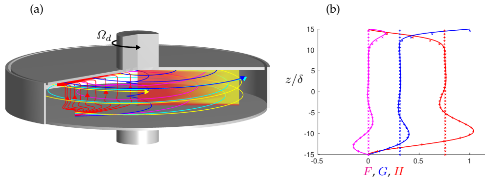
Figure 2: Rotor-stator flow in the inertial frame. (a) The meridional plan shows the azimuthal component of the velocity. Streamlines in the whole space (blue, magenta, cyan and yellow curves) and same streamlines restricted to a meridional plan (red curves). (b) Comparison between the Batchelor solution (solid curves) and the respective von Kármán (on the rotor above, marked by x symbols) and Bödewadt (on the stator below, marked by crosses) solutions. Axial shape functions F (magenta), G (blue) and H (red) of the velocity profile, as functions of z/\delta .
