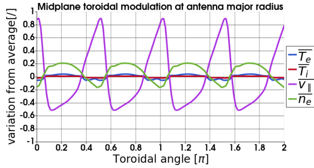
Figure 9: Relative midplane toroidal modulation of plasma physical quantities as defined in section 2. T_i and T_e varies along the toroidal direction from the average less than 0.05 times the max assumed value. The modulations are more important for n_e and v_{||} .
