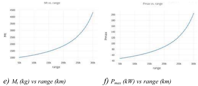
Fig. 4. Ustol configuration: simulation results for four passengers ( N_p=4 )
