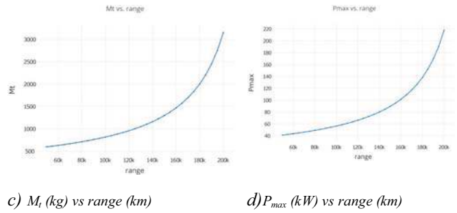
Fig. 3. Vtol configuration: simulation results for two passengers ( N_p=2 )
