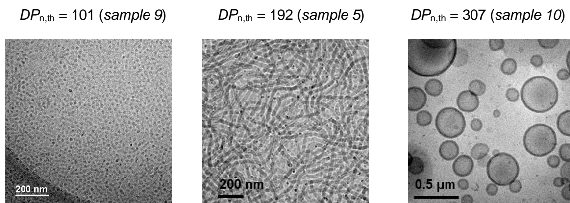
Figure 3. Representative cryo-TEM images of PDMAm 36 - b -P(CMAm- co -AA) samples synthesized with three different hydrophobic lengths at constant f_{AA,0} ( \sim 0.14 ) in acidic conditions. All samples were prepared at 1 wt% at room temperature in acidic water (0.03M HCl).
