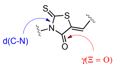
Figure 1. Geometric descriptors of 5-arylidene rhodanines d_{(C-N)} and \nu_{(C=O)} .
