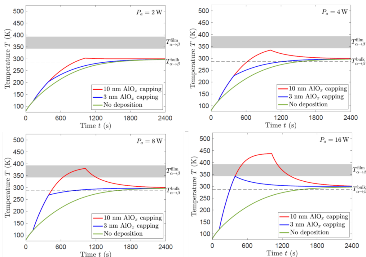
FIG. S12: Time evolution of the sample temperature during exposure to the AlO_x source thermal radiation for powers P_a indicated in the upper right corner of each graph.
