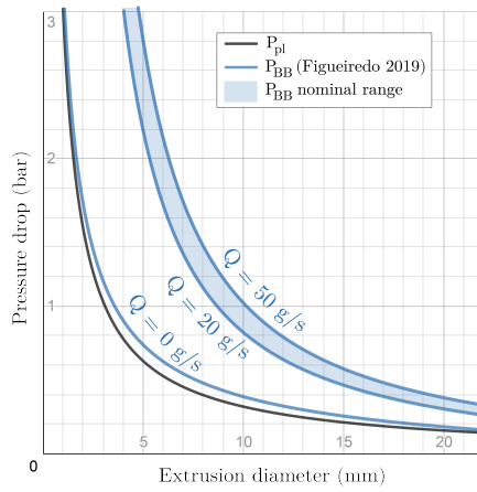
Figure 18: Pressure drop against output diameter for the velocity-independent case P_{Pl} and the velocity-dependant one P_{BB} . Parameter values from table 4, extracted from [21]. Flow rates between 20 and 50 g/s, l_p = 100\text{mm} .
