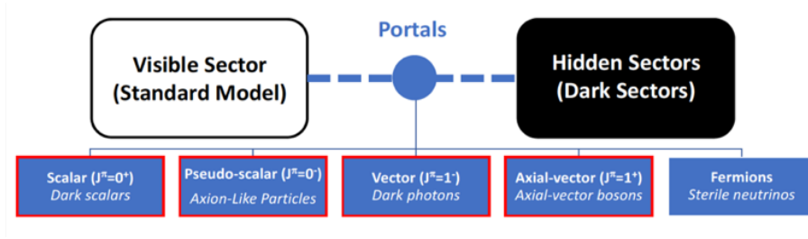
Figure 1. Illustration of the Standard Model coupling to Dark Sectors through given portals. Portals that might be studied through nuclear physics experiments are indicated with a red frame.
