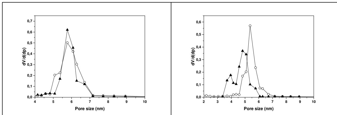
Figure 6. (Left) BJH pore size distribution of SBA-15-80 soaked into water (open circle) and OCP(CAN) 93 mg/g immobilized on SBA-15-80 under blue light (full triangle). (Right) BJH pore size distribution of SBA-15-80-NH 2 soaked into water (open circle) and OCP(CAN) 85 mg/g immobilized on SBA-15-80-NH 2 under blue light (full triangle).
