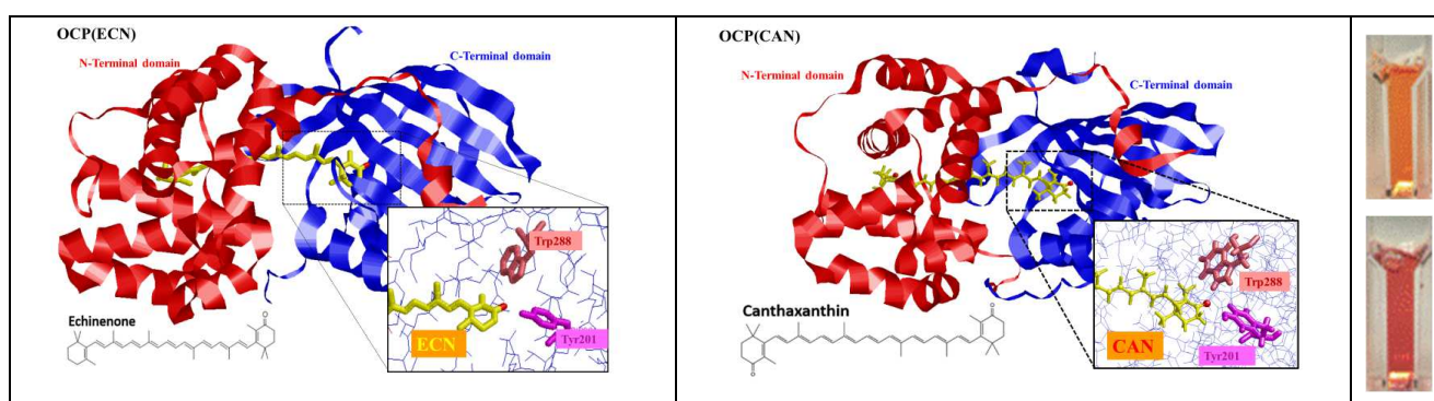
Figure 1. (Left) Crystal structure of OCP binding Echinonone from cyanobacteria Synechocystis PCC 6803 (PDB 3mg1 [7]). (Middle) Crystal structure of OCP binding Canthaxanthin from cyanobacteria Synechocystis PCC 6803 (PDB 4xb5 [8]). ECN and CAN are depicted in yellow in the 3D view, with oxygen atoms in red. In the bottom, left corner of each picture there is the chemical structure of ECN and CAN; in the bottom, right corner there is a zoom-in on interactions between the carbonyl group of carotenoids and amino acids Tyr201 and Trp288 belonging to the C-terminal domain. (Right) OCP in solution before photoactivation (OCP 0 ) (top) and OCP in solution after photoactivation (OCP R ) (bottom).
