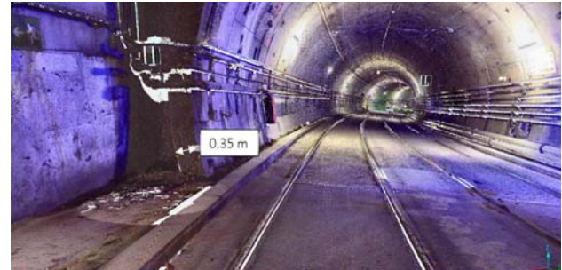
Fig. 5: View of the tunnel and measurement of the thickness of the voussoirs
