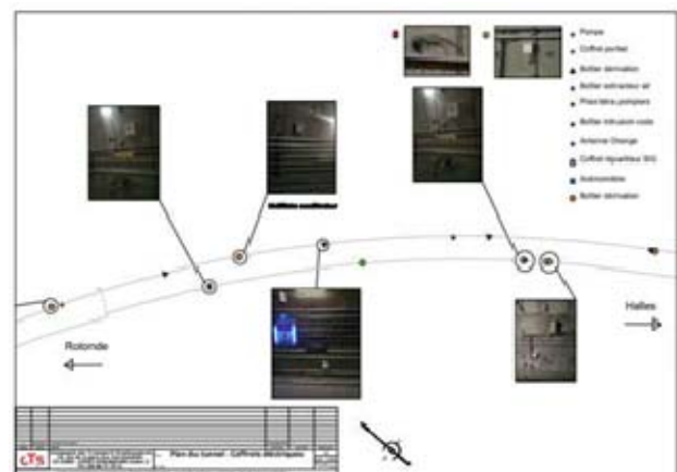
Fig. 6: 2D plan with implantation of technical units
