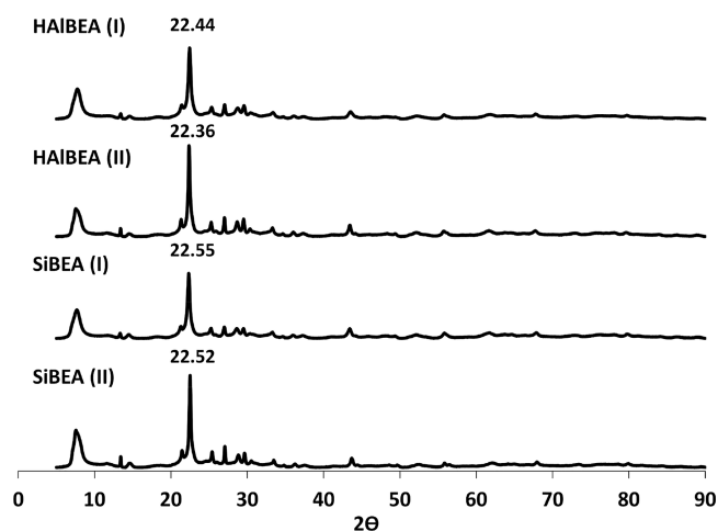
Figure 1. X-ray diffractograms of \text{SiBEA} (II), \text{SiBEA} (I), \text{HAIBEA} (II), and \text{HAIBEA} (I) zeolites.
