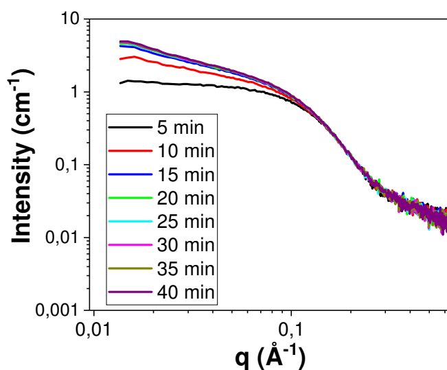
Figure S8. In situ SAXS patterns recorded during the partial reduction of \text{HAuCl}_4 \cdot 3\text{H}_2\text{O} using 0.5 eq. of TIPS at 40 °C ( [\text{Au}] = 20 \text{ mM} , [\text{TIPS}] = 10 \text{ mM} ).
