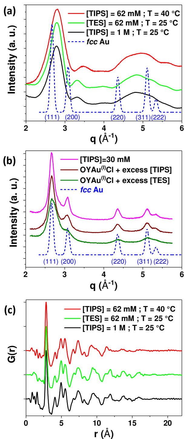
Figure 6. (a) In situ high-energy X-ray diffraction Au NPs prepared at T = 25 °C with [TES] = 62 mM (green line), [TIPS] = 1 M TIPS (black line) or at 40°C with [TIPS] = 62 mM (red line); (b) XRD pattern of Au NPs prepared using the stoichiometric amount of TIPS (30 mM) and by the direct reduction of the lamellar phase OY-Au(I)-Cl with a large excess of TIPS or TES; (c) G(r) oscillations of the Au NPs prepared at T = 25 °C with [TES] = 62 mM (green line), [TIPS] = 1 M TIPS (black line) or at 40°C with [TIPS] = 62 mM (red line). (a) and (b): q = \frac{4\pi \sin \theta}{\lambda} and the dash blue line corresponds to the theoretical XRD pattern of fcc Au with an arbitrary peak broadening.
