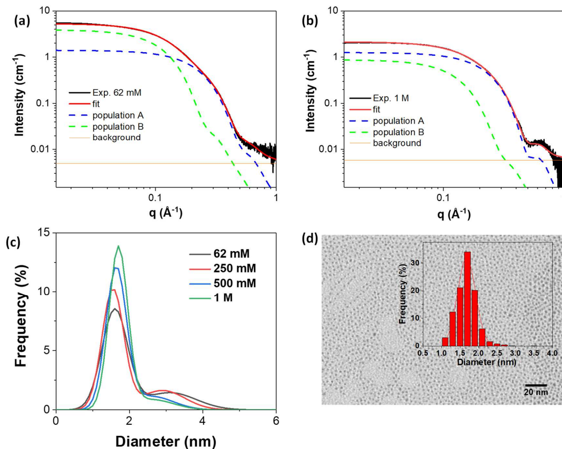
Figure 1. SAXS patterns of suspensions of Au nanoparticles obtained after 3h of reaction of HAuCl 4 .3H 2 O in OY/hexane ([Au] = 20 mM; [OY] = 50 mM) using TIPS as reducing agent, in different concentrations: (a) [TIPS] = 62 mM and (b) [TIPS] = 1 M. In black: experimental data; red: the corresponding fit considering two populations of nanospheres (blue and green dashed lines) and a constant background (orange) ; (c) volume-weighted distribution determined from the fit of the in situ SAXS of the final Au NPs obtained after 3h of reaction with different TIPS concentrations ; (d) TEM image of Au nanoparticles obtained after 3h of reaction at T = 25°C with [TIPS] = 1 M. Inset : the corresponding number-weighted size distribution determined from the image analysis.
