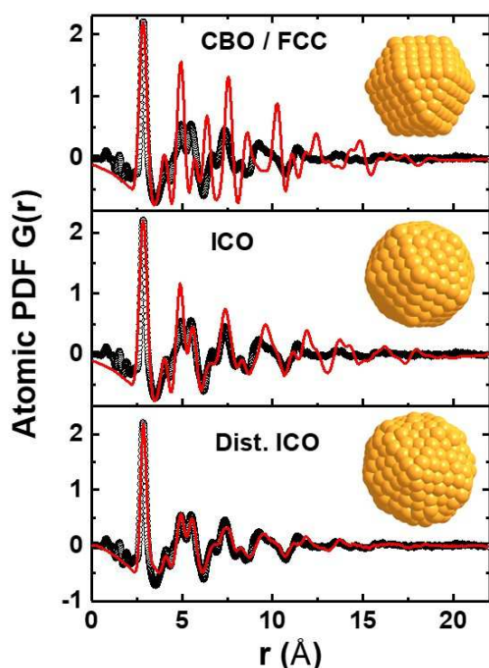
Figure 7. Comparison between experimental PDF of Au NPs prepared by reduction with [TIPS] = 62 mM at 40 °C (black circle) and different computed atomic PDFs (red line). CBO is a 309 atoms cuboctahedron with fcc structure, ICO is a 309 atoms icosahedron and Dist. ICO is a 435 atoms distorted icosahedron. Inset : images of the structural models. Both the CBO and the 309-atom ICO have a perfect structure rendering the atomic coordination spheres/PDF peaks sharp. Although larger in size than 309-atom models, the 435-atom ICO is distorted and so exhibits somewhat smeared coordination spheres/PDF peaks in comparison to perfect CBO and ICO polyhedral.
