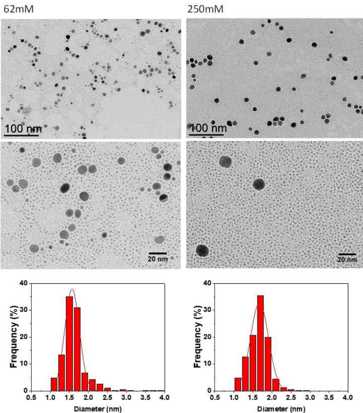
Figure S3. TEM images (1 st and 2 nd row) and the corresponding size distribution (3 rd row) of Au nanoparticles obtained after 3h of reaction for [TIPS] = 62 mM (left column) and 250 mM (right column). The large NPs have a very low occurrence compared to the small NPs and thus do not appear on the size distribution.
