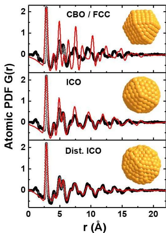
Figure S10. Comparison between experimental PDF of Au NPs prepared by reduction with [TES] = 62 mM at 25 °C (black circle) and different computed atomic PDFs (red line). CBO is a 309 atoms cuboctahedron with fcc structure, ICO is a 309 atoms icosahedron and Dist. ICO is a 435 atoms distorted icosahedron.
