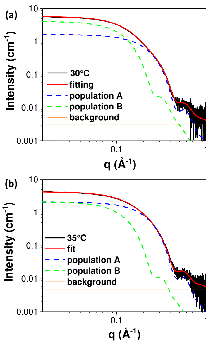
Figure S7. SAXS patterns of a suspension of Au nanoparticles prepared by reduction of \text{HAuCl}_4 \cdot 3\text{H}_2\text{O} in OY/hexane ( [\text{Au}] = 20 \text{ mM} ; [\text{OY}] = 50 \text{ mM} ) at 30°C and 35 °C using TIPS as reducing agent ( [\text{TIPS}] = 62 \text{ mM} ). Black: experimental data, red: best fits including two populations of nanospheres (A: dashed blue \sim 1.7 \text{ nm} ; B: dashed green \sim 3.5 \text{ nm} ) and a constant background (orange).
