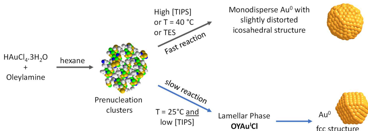
Figure 8. Schematics of the competition between the direct pathway leading to the crystallization of ultra-small Au NPs with the icosahedral structure and the one involving the lamellar phase OY-Au(I)-Cl and leading to bigger particles with the fcc structure.
