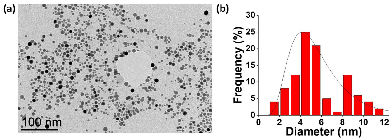
Figure S6. (a) TEM image of Au nanoparticles prepared with [TIPS] = 30 mM, i.e. in stoichiometric amount ; (b) Number-weighted size distribution determined from the TEM image analysis.
