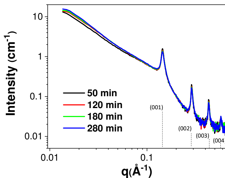
Figure S5. In situ SAXS of the lamellar phase OY-Au(I)-Cl recorded during the partial reduction of \text{HAuCl}_4 \cdot 3\text{H}_2\text{O} using 0.5 eq. of TIPS at 25 °C ( [\text{Au}] = 20 \text{ mM} , [\text{TIPS}] = 10 \text{ mM} ).
