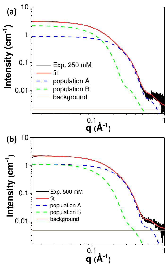
Figure S2. SAXS patterns of suspensions of Au nanoparticles obtained after 3h of reaction of \text{HAuCl}_4 \cdot 3\text{H}_2\text{O} in OY/hexane ( [\text{Au}] = 20 mM; [\text{OY}] = 50 mM) using TIPS as reducing agent: (a) [\text{TIPS}] = 250 mM and (b) [\text{TIPS}] = 500 mM. In black: experimental data; red: the corresponding fit considering two populations of nanospheres (blue and green dashed lines) and a constant background (orange).
