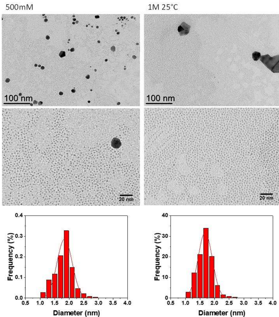
Figure S4. TEM images (1 st and 2 nd row) and the corresponding size distribution (3 rd row) of Au nanoparticles obtained after 3h of reaction for [TIPS] = 500 mM (left column) and 1 M (right column). The large NPs have a very low occurrence compared to the small NPs and thus do not appear on the size distribution
