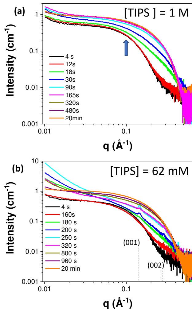
Figure 2. Time-resolved in situ synchrotron SAXS patterns recorded during the synthesis of Au nanoparticles in OY/hexane solution with different TIPS concentrations: (a) [TIPS] = 1M (the arrow indicates the “knee-position” on the SAXS at 4s. The knee is shifted to high q after 18 s; (b) [TIPS] = 62 mM. Dashed lines point the (00 l ) peaks of a lamellar phase with an interlayer distance d_{001} = 43.5 \text{ \AA} .
