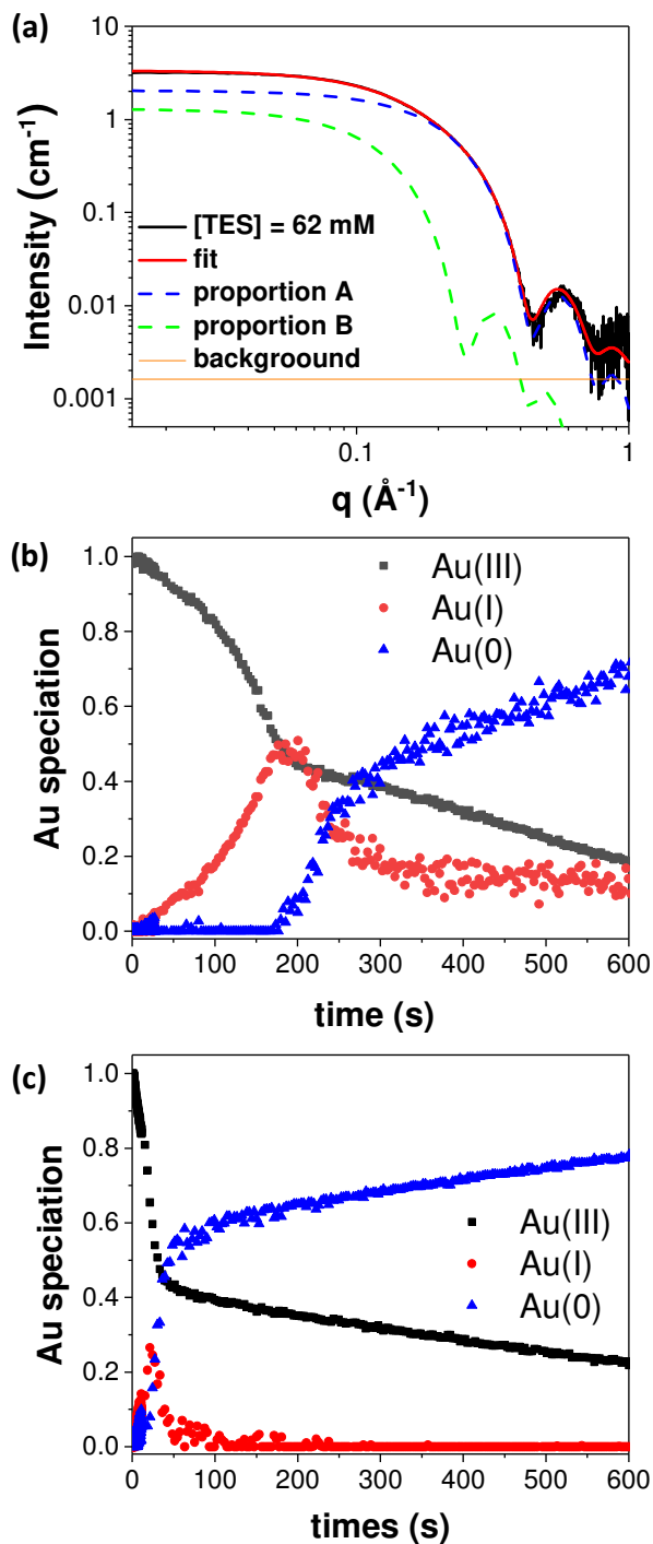
Figure 5. (a) SAXS pattern of Au nanoparticle prepared at 25°C using TES as reducing agent ([TES] = 62 mM); (b-c) Relative Au(III), Au(I) and Au(0) concentrations deduced from the linear combination analysis of the XAS spectra measured in situ during the reaction using (b) [TIPS] = 62 mM and (c) [TES] = 62 mM as reducing agent.
