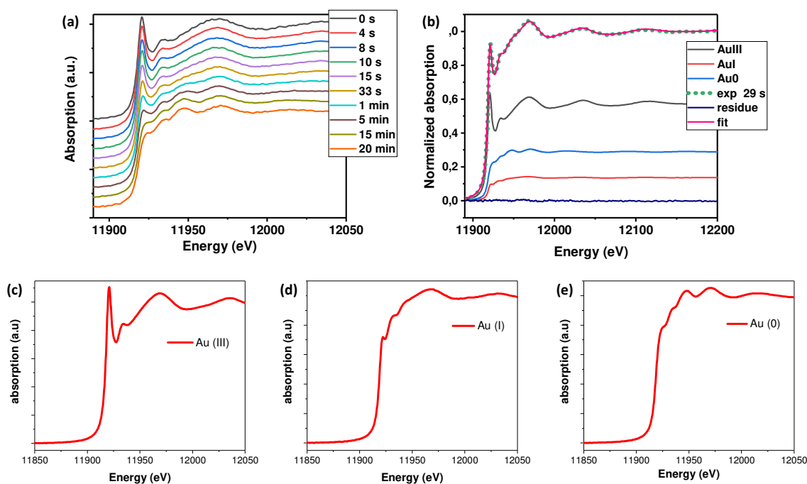
Figure S9. (a) In situ XAS spectra at the Au L_{III} -edge recorded during the reduction of \text{HAuCl}_4 \cdot 3\text{H}_2\text{O} in OY/hexane ( [\text{Au}] = 20\text{ mM} ; [\text{OY}] = 50\text{ mM} ) with [\text{TES}] = 62\text{ mM} ; (b) Fit of the XAS spectrum at 29 s (open circle) by a linear combination of three components (magenta line): Au(III) precursor (black), Au(I) intermediate (red) and the final Au(0) NPs (blue); (c) In situ XAS spectra at the Au L_{III} -edge of the precursor solution containing 20 mM \text{HAuCl}_4 \cdot 3\text{H}_2\text{O} and 50 mM in hexane; (d) In situ XAS spectra at the Au L_{III} -edge of the lamellar phase OY-Au(I)-Cl in suspension in hexane; (e) Au nanoparticles prepared by reduction of the precursor solution with a large excess of TIPS.
