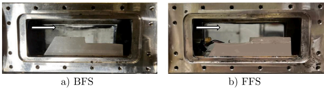
Fig. 19. Paraffin slabs mounted in the combustion chamber.
