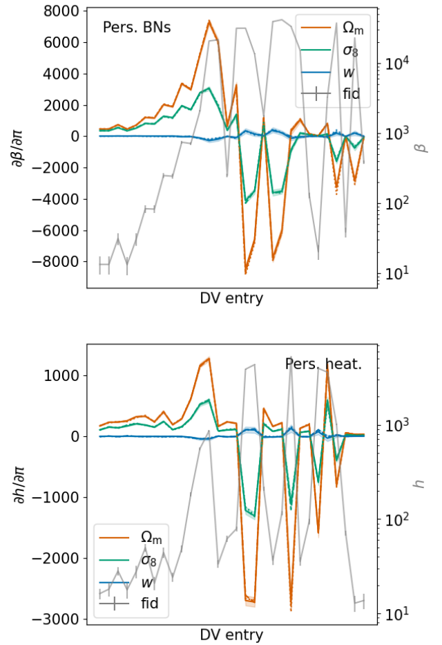
Fig. 13. Fiducial DV (gray) along with its derivatives with respect to \Omega_m (orange), \sigma_8 (green), and w (blue) for pers. BNs (top) and pers. heat. (bottom) computed on aperture mass maps from \gamma , smoothed with a 2:34 Schirmer et al. (2007) filter. The x -axis corresponds to compression coefficients with no physical meaning.
