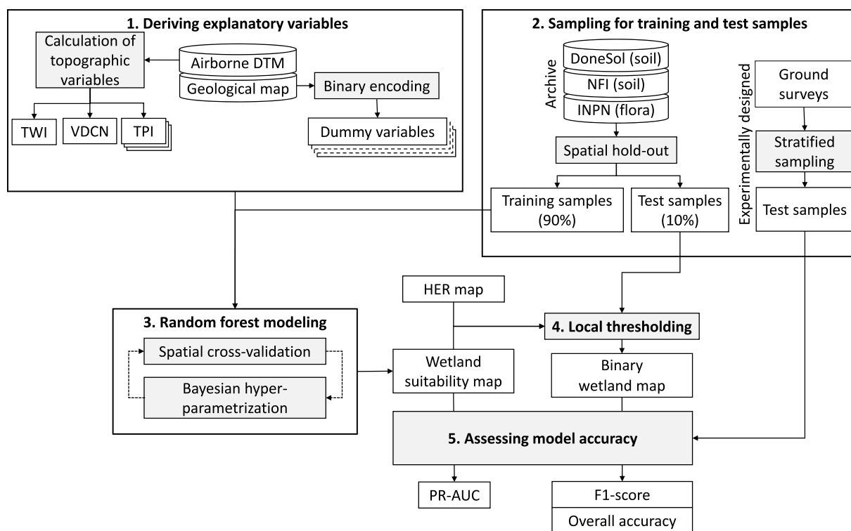
Fig. 3. Flowchart of the method used to map wetlands by modeling topographic and geological variables subsequently calibrated and validated using soil and flora field samples.
