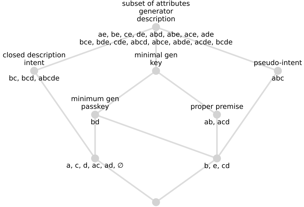
Figure 2: The concept lattice of “characteristic attribute sets” of the context introduced in Table 1.
