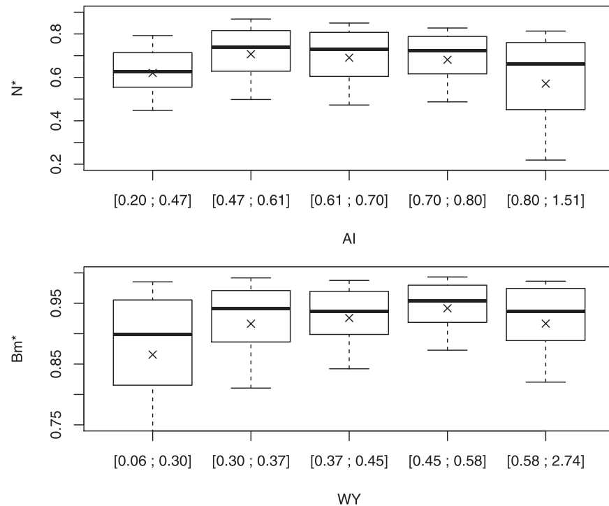
Figure 8. Impact of the aridity index ( AI ) on high-flow efficiency ( N* ) and of water yield ( WY ) on water balance reproduction ( Bm* ).
