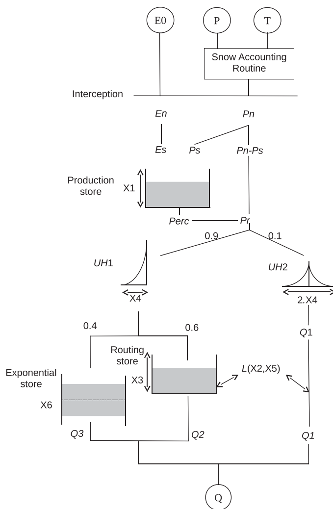
Figure 2. Schematic representation of the GR6J hydrological model with E_0 potential evapotranspiration, P precipitation, T temperature, Q streamflow. The letter X ( X_1, \dots, X_6 ) refers to the model parameters. The other letters ( P_n, E_n, \dots ) refer to internal variables, i.e., the water quantities exchanged between the reservoirs. A complete description of the model equations can be found in Pushpalatha et al. [2011].
