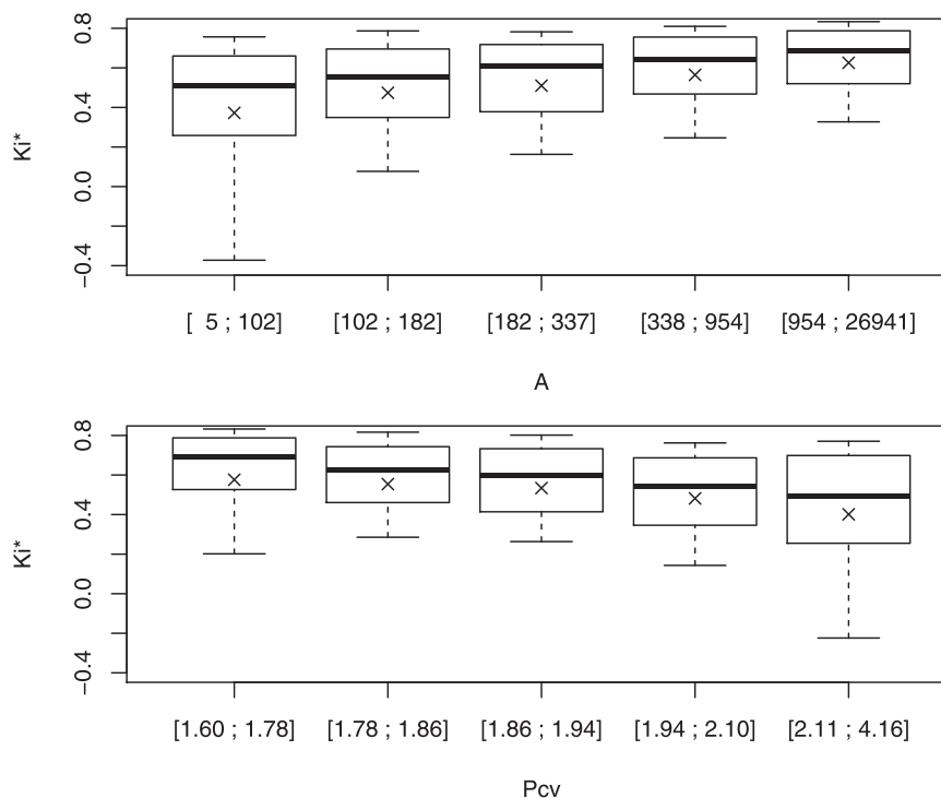
Figure 5. Impact of catchment area ( A ) and variation of precipitation ( Pcv ) on low-flow simulation. According to the design of the one-dimensional analysis, the catchment set is ranked by increasing feature values and then divided into five classes composed of an equal number of catchments.
