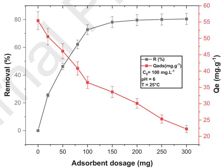
Fig.7. Effect of the adsorbent dosage on the adsorption of nitrate onto MgZnCoAl-C.
