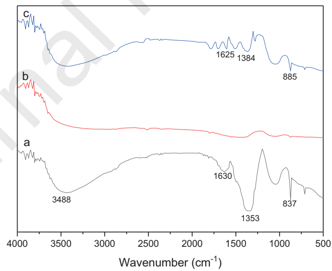
Fig.3. FTIR spectra for (a) MgZnCoAl- \text{CO}_3 , (b) MgZnCoAl-C, (c) MgZnCoAl- \text{NO}_3
