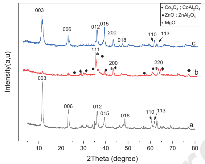
Fig.2. XRD patterns of (a) MgZnCoAl- \text{CO}_3 ; (b) MgZnCoAl-C; (c) MgZnCoAl- \text{NO}_3^-
