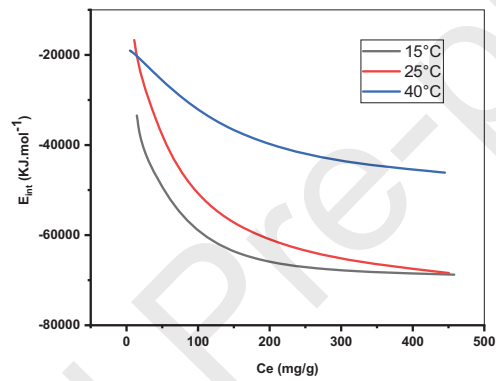
Fig.17. Evolution of the Internal Energy relative to the sorption system at 15 °C, 25 °C and 40°C .
