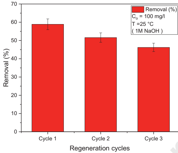
Fig.18: Regeneration study for MgZnCoAl-C at 1M NaOH
