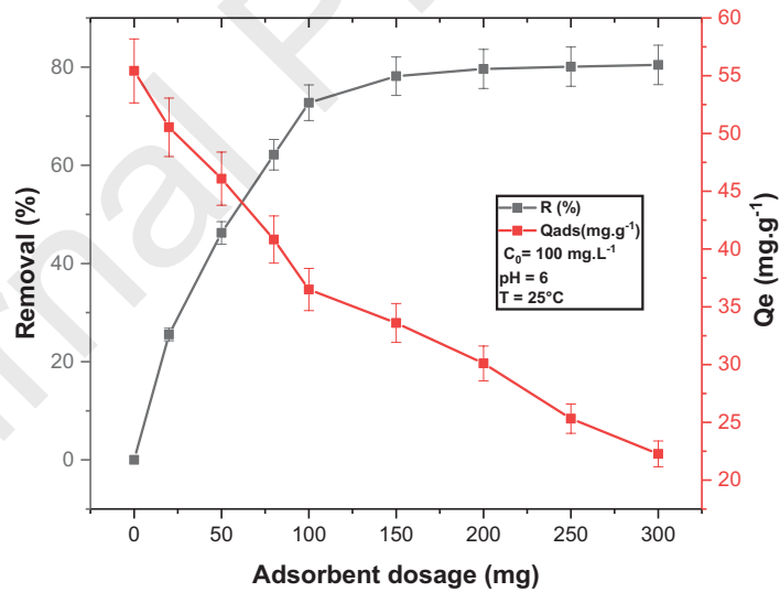
Fig.7. Effect of the adsorbent dosage on the adsorption of nitrate onto MgZnCoAl-C.
