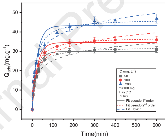
Fig 9. The curves representative of Nonlinear simulation of the pseudo-first-order (PFO), pseudo-second-order (PSO), and Elovich
