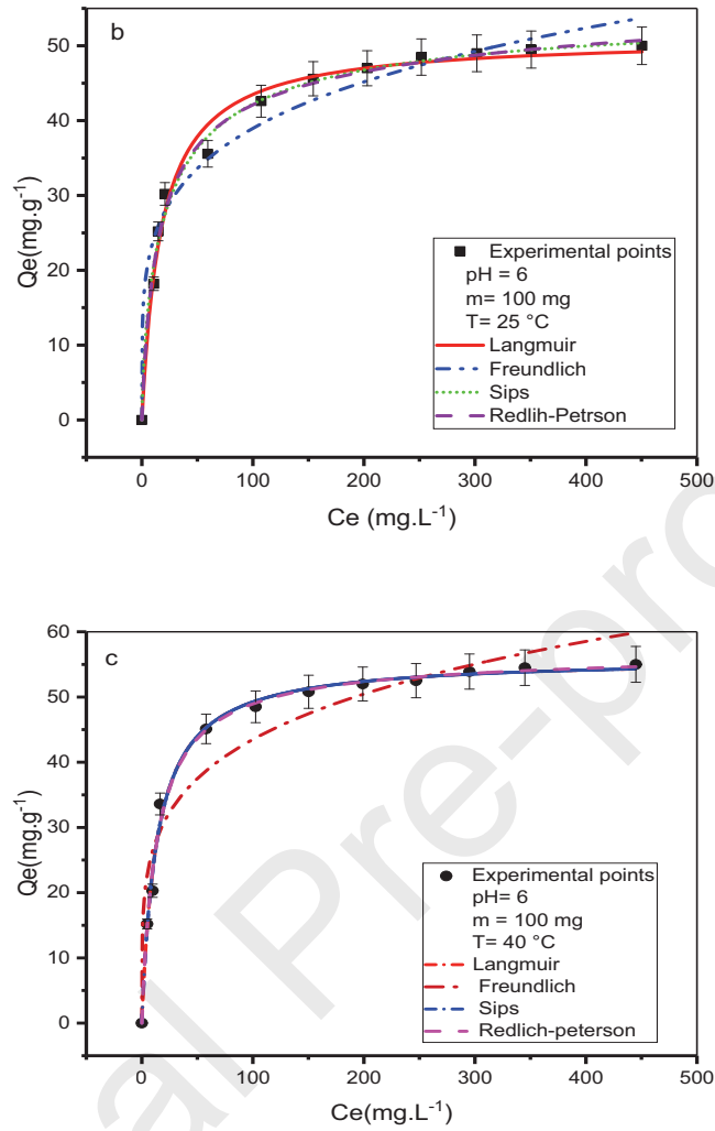
Fig.11. Adsorption isotherms, (a) 15 °C, (b) 25 °C, and (c) 40 °C
