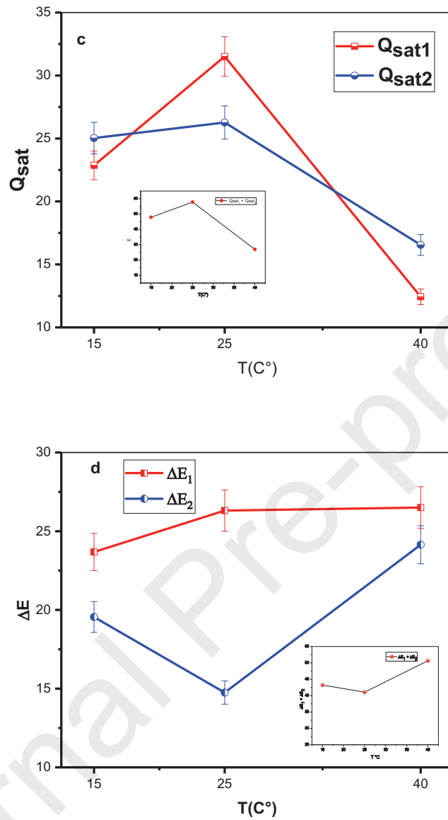
Fig 13: a) n_1 and n_2 versus temperature for the adsorption of \text{NO}_3 ; b) N_{m1} and N_{m2} versus temperature for the adsorption of \text{NO}_3 ; c) Q_{\text{sat}1} and Q_{\text{sat}2} versus temperature for the adsorption of \text{NO}_3 ; d) Estimated adsorption energies for nitrate removal.
