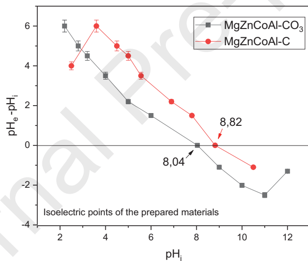
Fig.1. Isoelectric points of the prepared materials.
