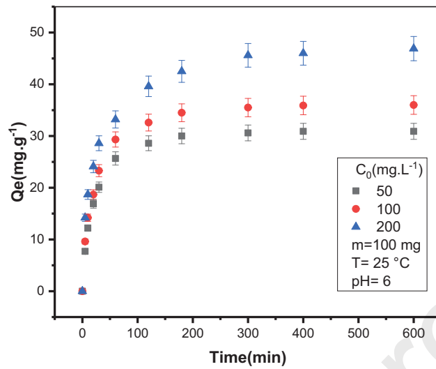
Fig. 8. Effect of contact time and initial nitrate concentrations onto MgZnCoAl-C
