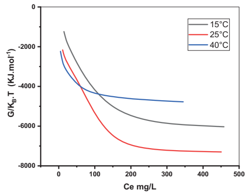
Fig.16. Evolution of the Gibbs Free Enthalpy at 15, 25, and 40 °C.
