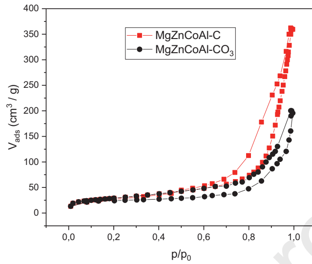
Fig.4. Adsorption/desorption isotherms of MgZnCoAl-CO 3 and MgZnCoAl-C.
