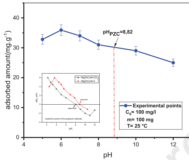
Fig 6. Effect of initial pH on adsorption of nitrate onto MgZnCoAl-C sample.
