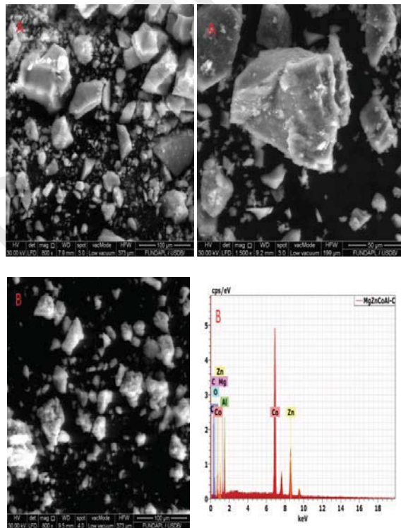
Fig . 5 .SEM micrographs of (A) MgZnCoAl-CO 3 (B) MgZnCoAl-C
