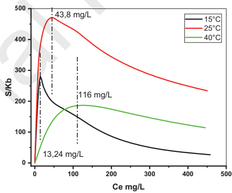
Fig. 15. Entropy as a feature of Ce at 15, 25, and 40 °C.
