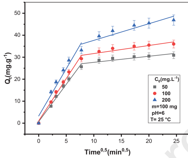
Fig.10. Data fitting of the nitrate adsorption kinetics by intra-particle diffusion model onto MgZnCoAl-C at different concentrations.
