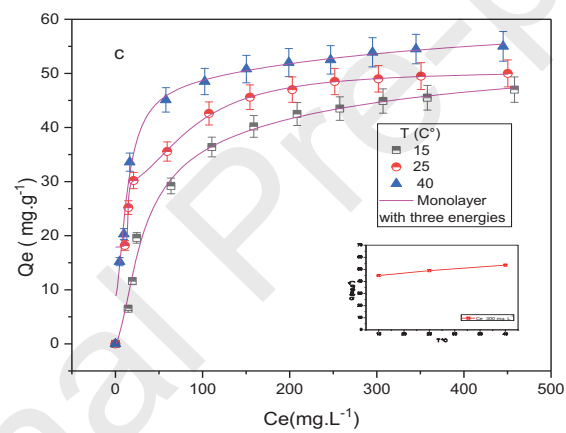
Fig 12: Data fitting of the nitrate adsorption isotherm by a) Monolayer with one binding site; b) Monolayer with two binding site; c) Monolayer with three binding site.
