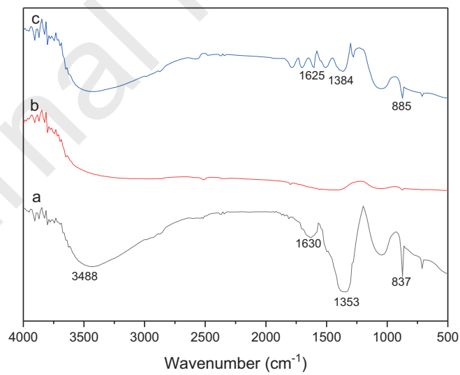
Fig.3. FTIR spectra for (a) MgZnCoAl-CO 3 , (b) MgZnCoAl-C, (c) MgZnCoAl-NO 3
