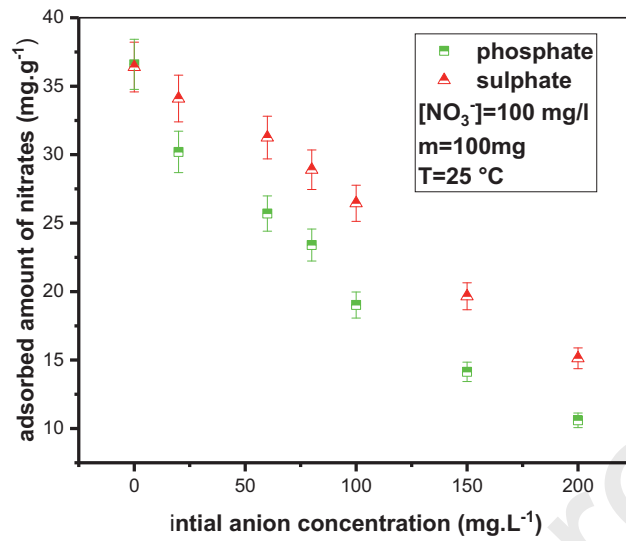
Fig.14. Adsorbed amount of versus initial anion concentration of solution with initial nitrate concentration of 100 mg/L.
