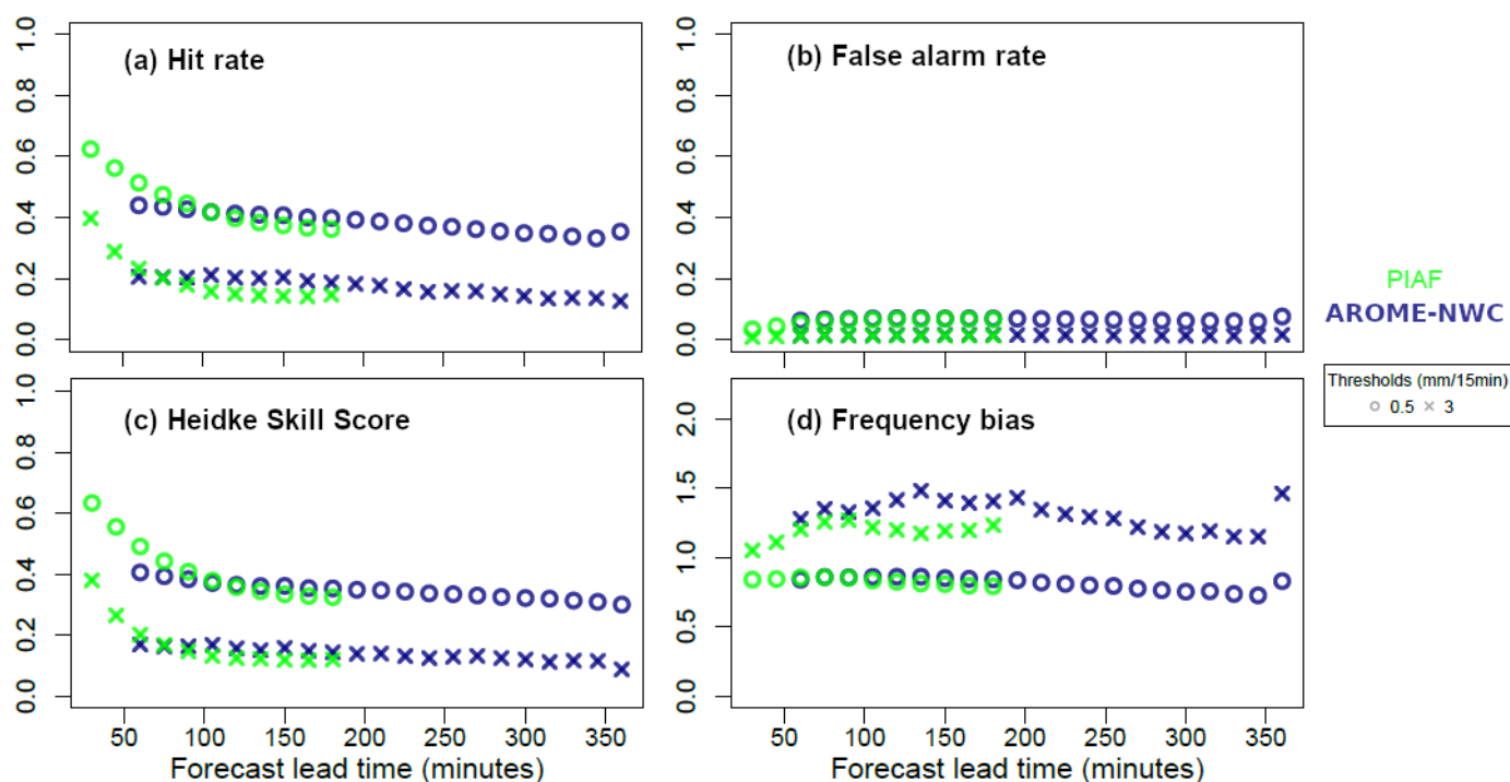
Figure 4. (a) Hit rate, (b) false alarm rate, (c) Heidke Skill Score, and (d) frequency bias for thresholds: 0.5mm/15min and 3mm/15min computed for AROME-NWC (in blue) and PIAF (in green) over their respective forecast ranges for 15-min rain accumulation over the box displayed Figure 1.
