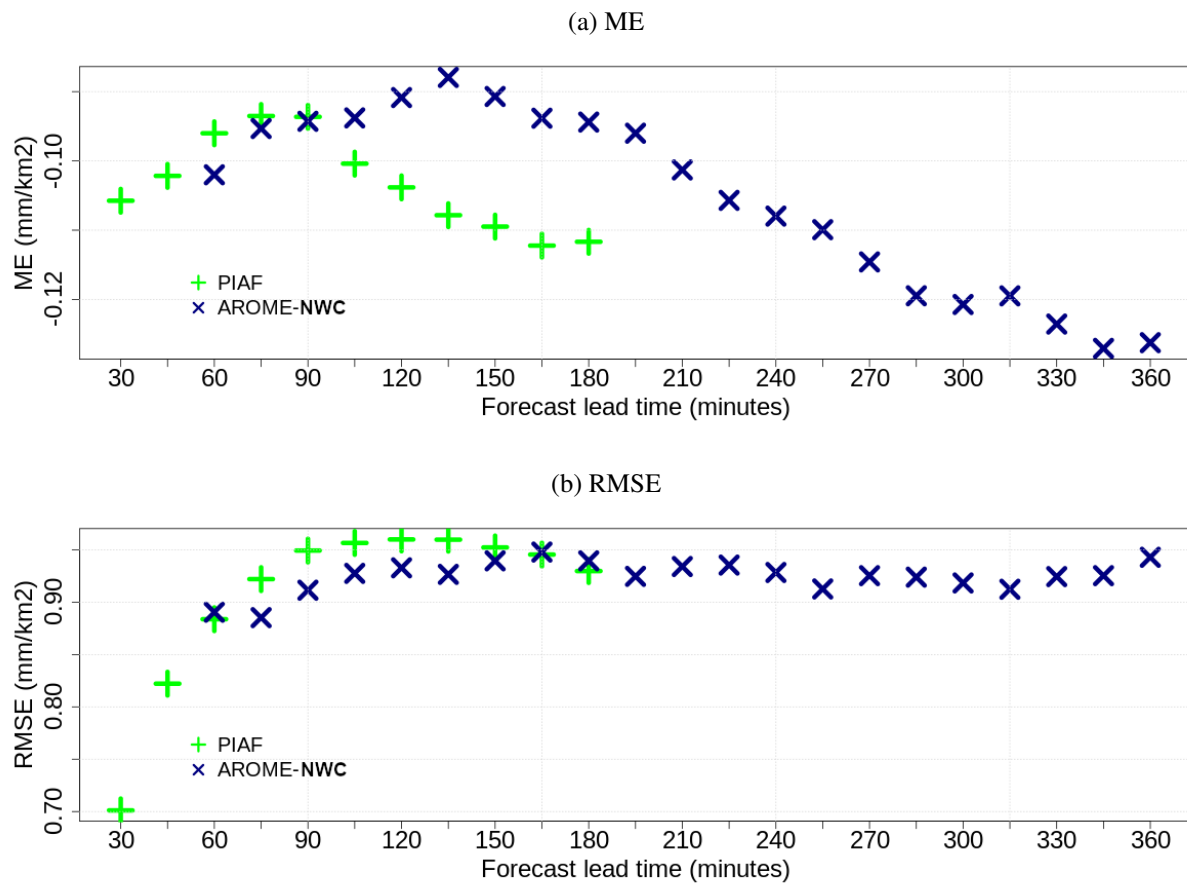
Figure 3. (a) Mean and (b) root mean square errors for AROME-NWC (in blue) and PIAF (in green) over their respective forecast ranges for 15-min rain accumulation forecasts. Scores computed over the box displayed Figure 1.
