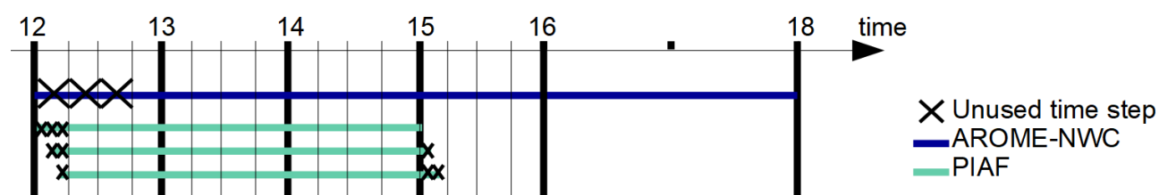
Figure 2. Example showing the unused time steps for a AROME-NWC forecast run starting at 1200 UTC and for three successive PIAF forecasts starting at 1200, 1205 and 1210 UTC.
