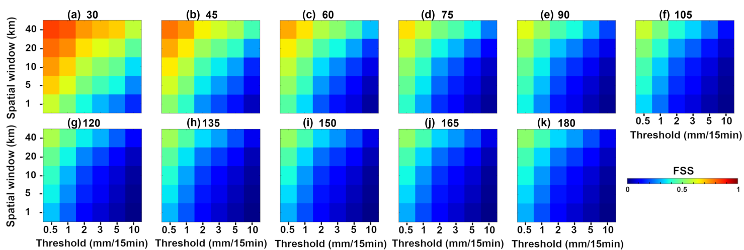
Figure 6. The 10-events mean FSS obtained with PIAF for the different precipitation thresholds (0.5, 1, 2, 3, 5 et 10 mm/15min) and window sizes (1, 5, 10, 20 et 40 km) at each forecast lead time from (a) 30 min to (k) 180 min.
