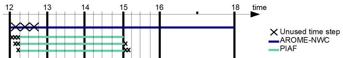
Figure 2. Example showing the unused time steps for a AROME-NWC forecast run starting at 1200 UTC and for three successive PIAF forecasts starting at 1200, 1205 and 1210 UTC.
