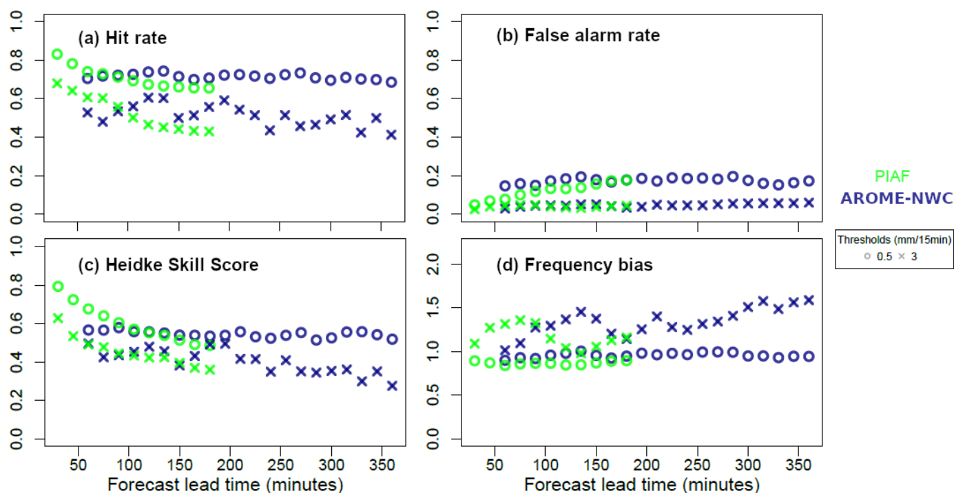
Figure 9. (a) Hit rate, (b) false alarm rate, (c) Heidke Skill Score, and (d) frequency bias for thresholds: 0.5mm/15min and 3mm/15min computed for AROME-NWC (in blue) and PIAF (in green) over their respective forecast ranges for 15-min rain accumulation forecasts averaged over the catchments.
