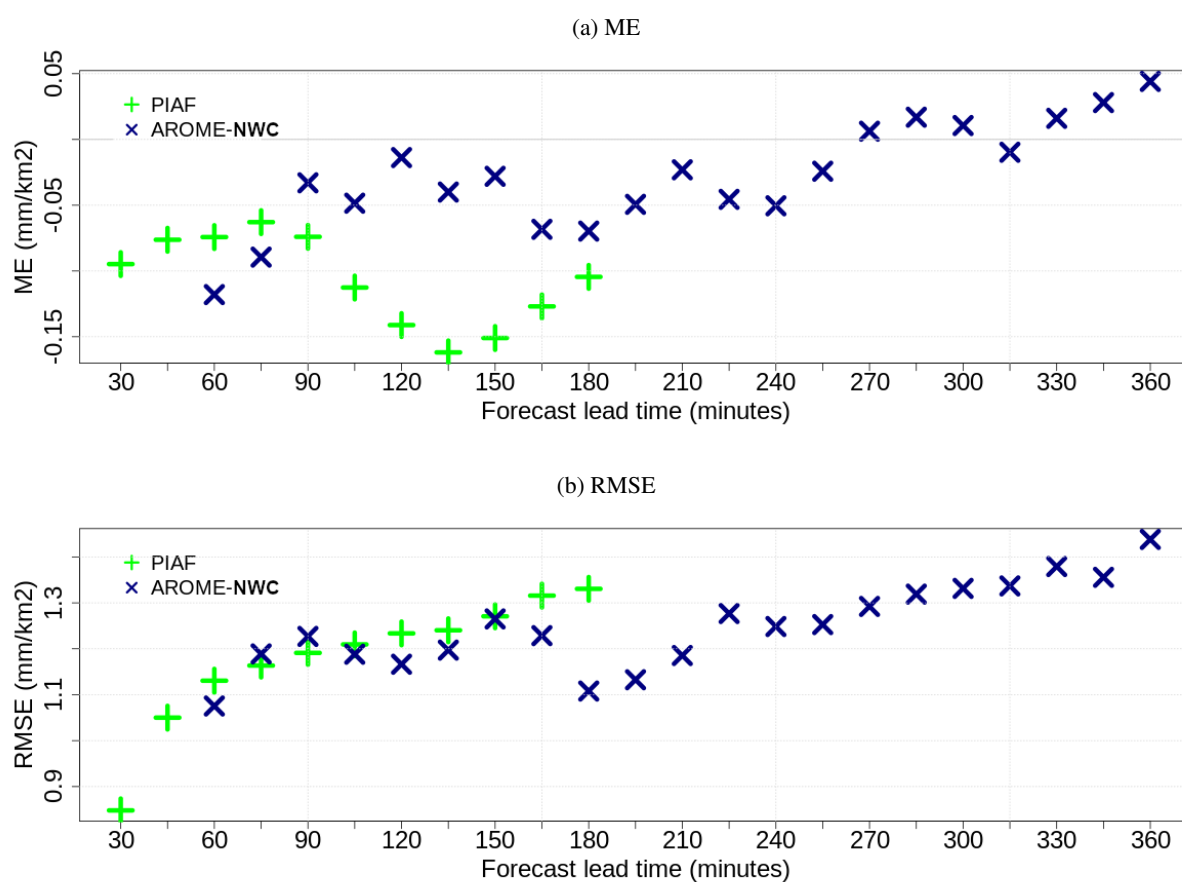
Figure 7. (a) Mean and (b) root mean square errors for AROME-NWC (in blue) and PIAF (in green) over their respective forecast ranges for 15-min rain accumulation forecasts averaged over the catchments.
