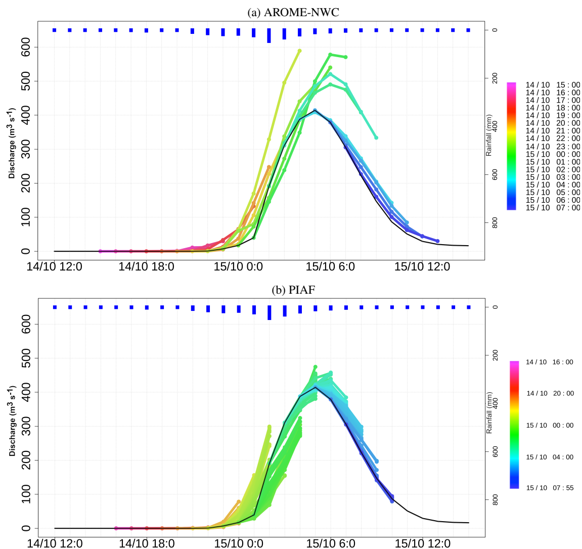
Figure 10. Discharge time series simulated by ISBA-TOP driven by ANTILOPE (black curve), by (a) AROME-NWC and by (b) PIAF for the case 15/10/2018 for the Orbiel river at Bouilhonnac (watershed No. 4). The reverse histogram represents the ANTILOPE hourly rainfall averaged over the catchment.
