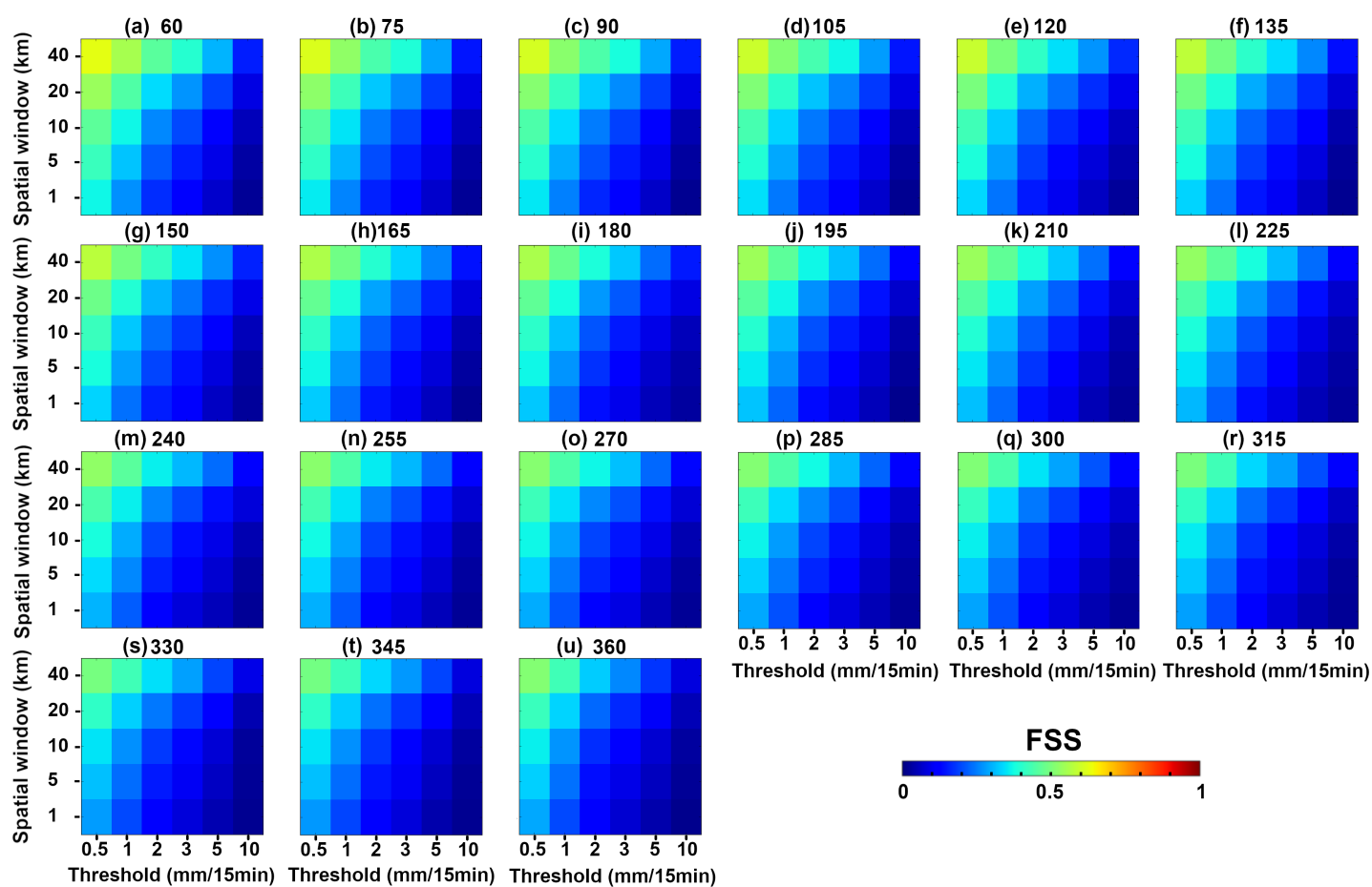
Figure 5. The 10-events mean FSS obtained with AROME-NWC for the different precipitation thresholds (0.5, 1, 2, 3, 5 et 10 mm/15min) and window sizes (1, 5, 10, 20 et 40 km) at each forecast lead time from (a) 60 min to (u) 360 min.
