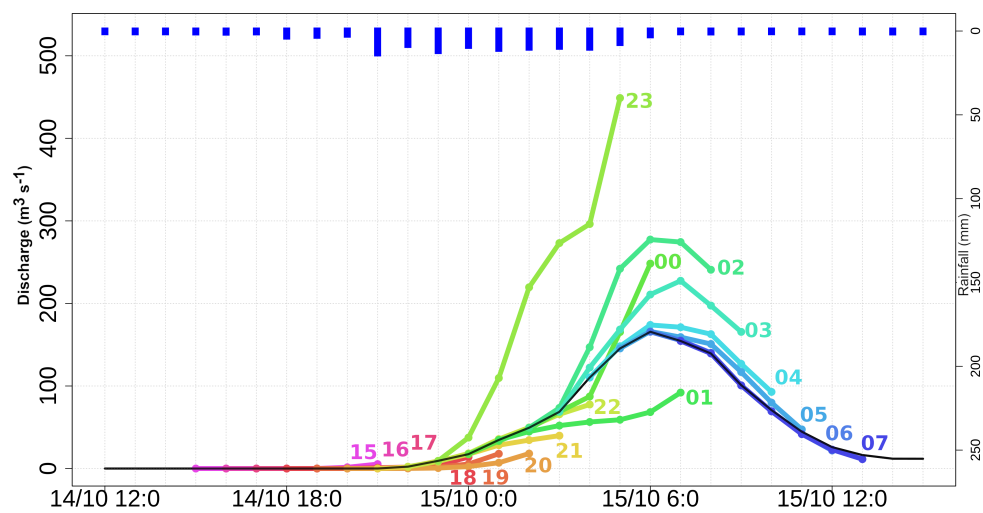
Figure 11. Discharge time series simulated by ISBA-TOP driven by ANTILOPE rainfall estimates (black curve) and by AROME-NWC forecasts (coloured curves with forecasts starting from 14 October 15 UTC to 15 October 07 UTC) for the Fresquel river at Pezens (watershed No. 1). The reverse histogram represents the ANTILOPE hourly rainfall averaged over the catchment.
