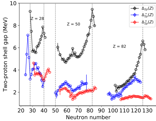
Fig. 3 Two-proton empirical shell gap computed in the three variants discussed in this work, namely \Delta_{2p}^- , \Delta_{2p}^+ and \Delta_{2p}^0 . Data are taken from the AME2020 [2]. Neutron magic numbers are marked by a dashed line.
