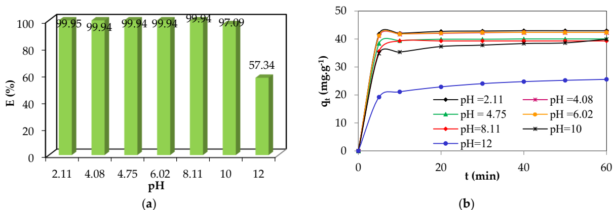
Figure 5. Evolution of the percentage removal (a) and amount adsorbed of phenol (b) at equilibrium as a function of the pH of the solution ( r = 0.6 \text{ g.L}^{-1} , T = 20 \text{ }^\circ\text{C} , C_0 = 25 \text{ mg.L}^{-1} , w = 300 \text{ rpm} ).
