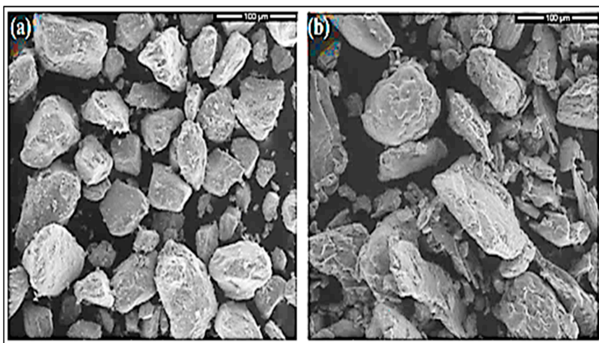
Figure 3. SEM image of raw WNSp (a) before and (b) after MBD adsorption (100 µm, 800×, 10 kV).
