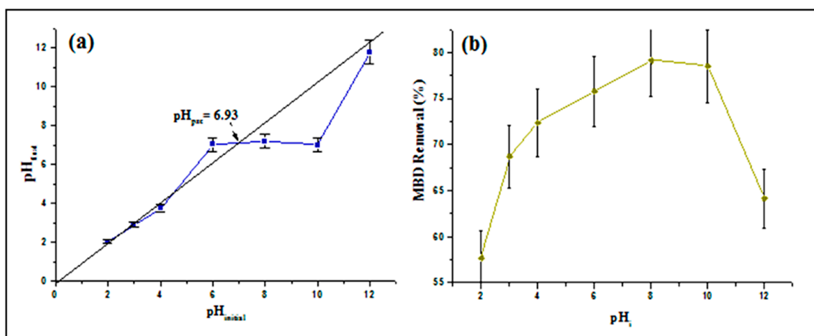
Figure 5. (a) pH at point of zero charge ( \text{pH}_{\text{pzc}} ), and (b) effect of pH on MBD adsorption.
