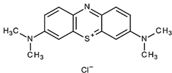
Figure 1. Chemical structure of methylene blue dye.
