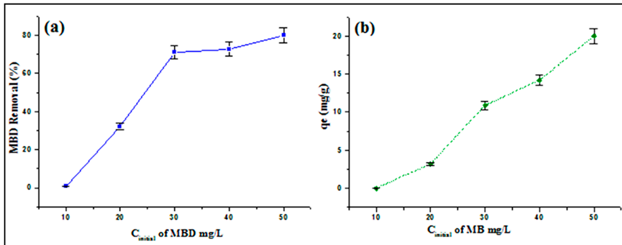
Figure 7. (a) Effect of the initial MBD concentration on MBD removal and (b) on the adsorption capacity of raw WNSp.
