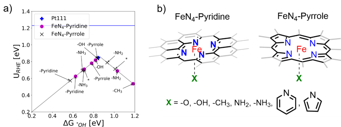
Figure 7. ORR activity volcano represented by O 2 reduction potential (RHE), U RHE , based on *OH binding energies (ΔG* OH ) simulated on a series of FeN 4 pyridine and pyrrole sites with different axial ligands, and compared with Pt(111) (a). Schemes showing axial coordination in FeN 4 -Pridine (left) and FeN 4 -Pyrrole (right), where X denotes the axial ligand (b). -* denotes a pristine FeN 4 structure.
