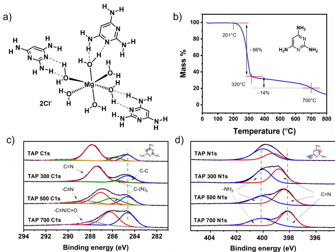
Figure 1. Representation of the self-assembly between 2,4,6-Triaminopyrimidine and MgCl 2 ·6H 2 O (a). TGA curve of TAP (b). C1s (c) and N1s (d) XPS spectra of TAP pyrolyzed at 300, 500, and 700 °C.
