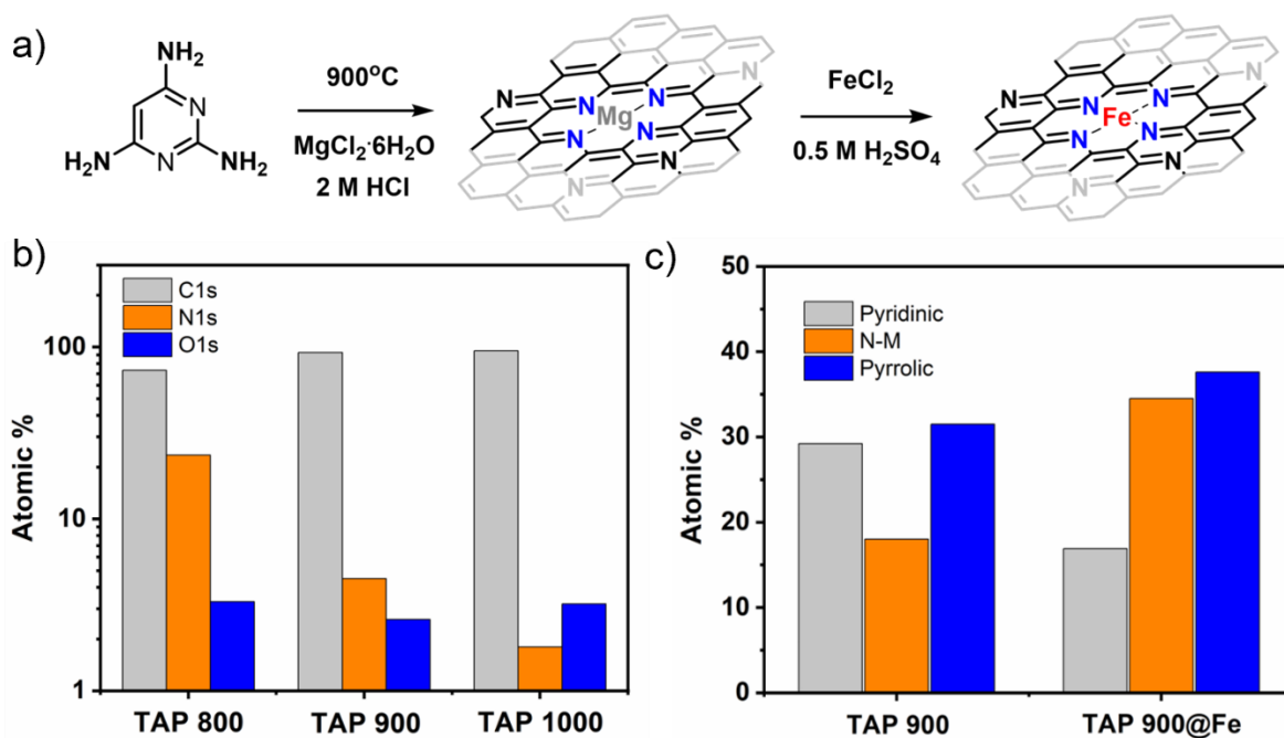
Figure 3. Schematic representation of Fe coordination in TAP-derived materials (a). Elemental composition of TAP-derived materials obtained by XPS plotted in a logarithmic scale (b) and decomposition of XPS N1s species in TAP 900 and TAP 900@Fe (c).
