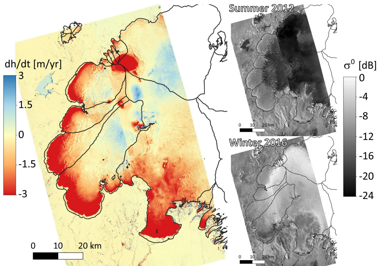
Figure 5: Surface elevation change rate [ m/yr ] over Vatnajökull Ice Cap (Iceland) from TanDEM-X bistatic acquisitions in summer 2012 and winter 2016. The right panels show the backscatter images [ dB ] for these two periods, illustrating the strong seasonal contrast and the need for correcting the varying radar penetration into snow and firn. A larger penetration depth is expected in the cold winter snow and firn (high backscatter) compared to the wet summer firn (low backscatter).
