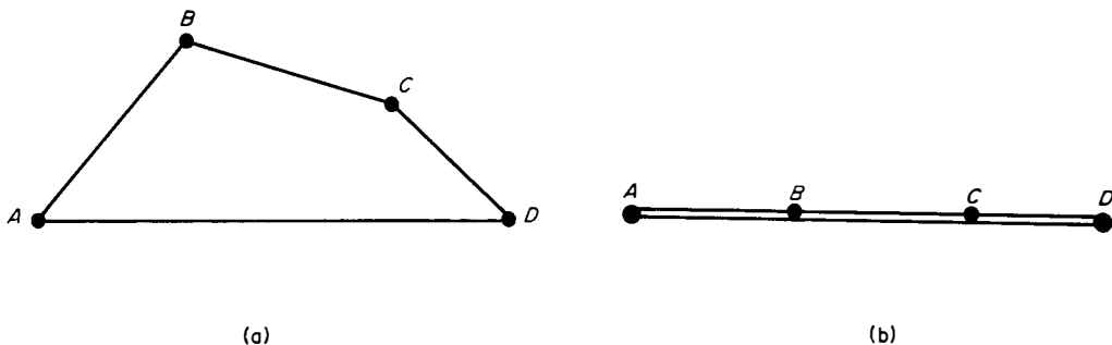
Fig. 6. A simple two-dimensional frame which has a single mode in configuration (a) but two (infinitesimal) modes—and a corresponding state of prestress—in configuration (b).
