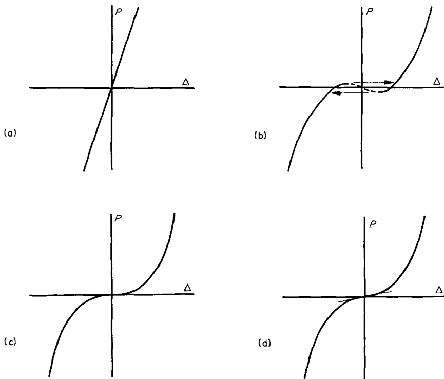
Fig. 5. Force ( P ), displacement ( \Delta ) relation for joint I of the frames of Figs. 2 (and 4). (a) "Normal" case, Fig. 2(a); the P , \Delta relation is linear. (b) The radial bars are a little longer than those which would meet at I in a plane. The P , \Delta relationship is a cubic, with two turning-points marking the ends of a zone of unstable equilibrium (-----), and snap-through into an inverted configuration can occur ( \rightarrow ). The origin is at the point corresponding to the (unstable) flat configuration. The linear curve of (a) corresponds to a short section of this curve on the left near the \Delta axis. (c) The radial bars are exactly the length to intersect at I in a plane. The P , \Delta relationship is P = \text{constant} \cdot \Delta^3 , and the slope is zero at the origin. (d) The radial bars are a little shorter than in case (c), and prestress is required to assemble the frame. The P , \Delta relationship of (c) is augmented by a linear term, which has the effect of "tilting" it. Note that curve (b) has tilt in the opposite sense.
