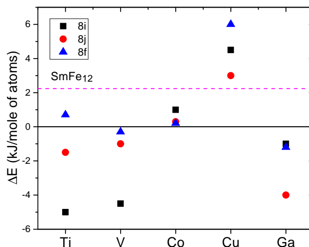
Figure 11. Calculated formation energy for \text{SmFe}_{11}M ( M = \text{Ti}, \text{V}, \text{Co}, \text{Cu}, \text{Ga} ) [113]. The magenta dashed line corresponds to formation energy of the hypothetical \text{SmFe}_{12} energy.
