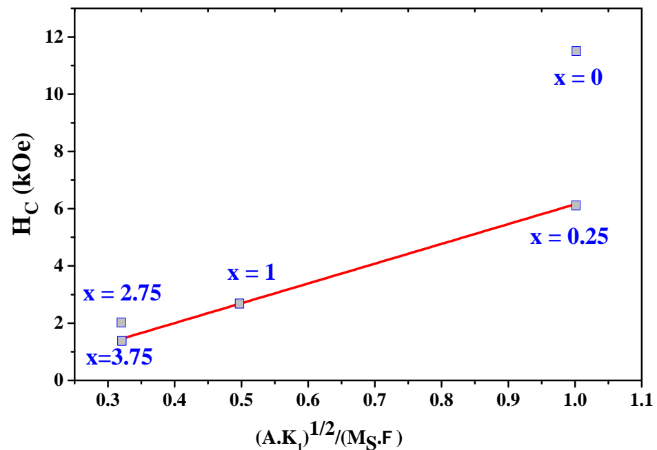
Figure 11. The experimental data on the coercivity H_c as a function of \zeta = (AK_1)^{1/2} .
