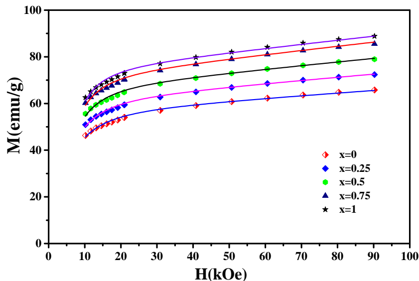
Figure 10. The magnetization curves M(H) of the nanocrystalline \text{Pr}_2\text{Co}_7\text{C}_x compounds ( x = 0, 0.25, 0.5, 0.75, \text{ and } 1 ). The solid lines show the fit to the experimental data (symbols).
