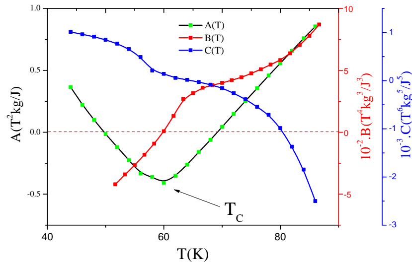
Figure 7. Landau parameter A(\text{T}^2\text{kg}/\text{J}) (black y -axis), B(\text{T}^4\text{kg}^3/\text{J}^3) (red y -axis), and C(\text{T}^6\text{kg}^5/\text{J}^5) (blue y -axis) plotted against temperature around the T_C for \text{SmNi}_3 sample.
