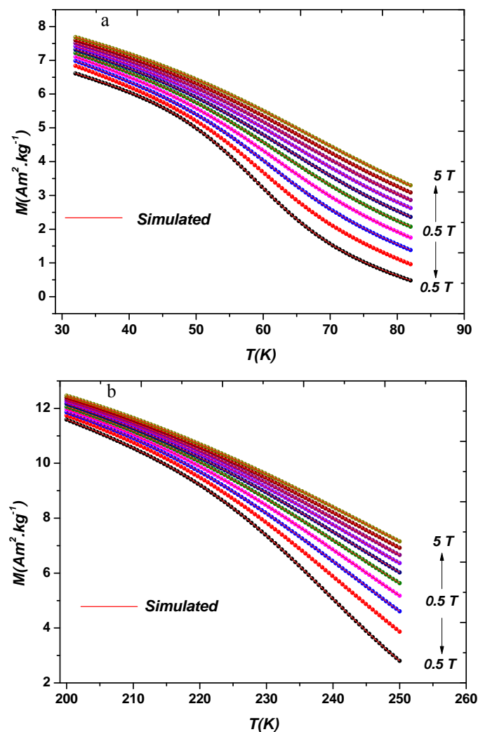
Figure 9. Magnetization vs. temperature for \text{SmNi}_3 (a) and \text{SmNi}_{2.2}\text{Fe}_{0.8} (b) under several magnetic fields.
