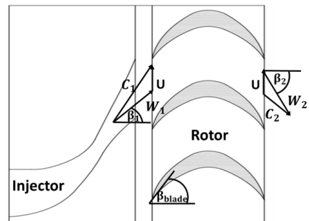
Figure 3. Scheme of the turbine
