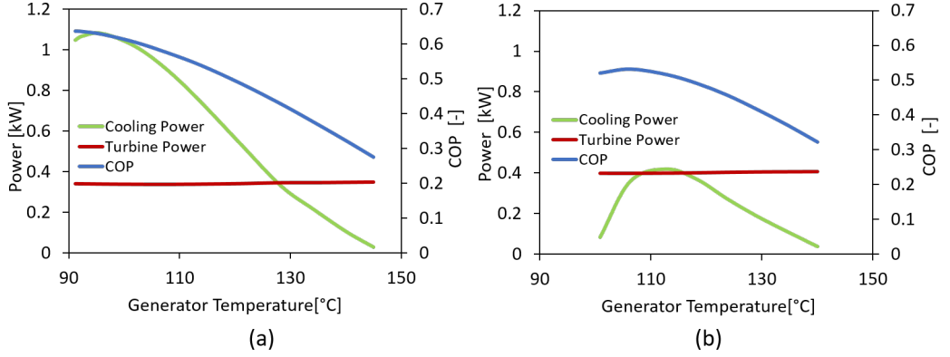
Figure 7. Generator Temperature influence for a cooling production at 5°C (a) and -5°C (b)
