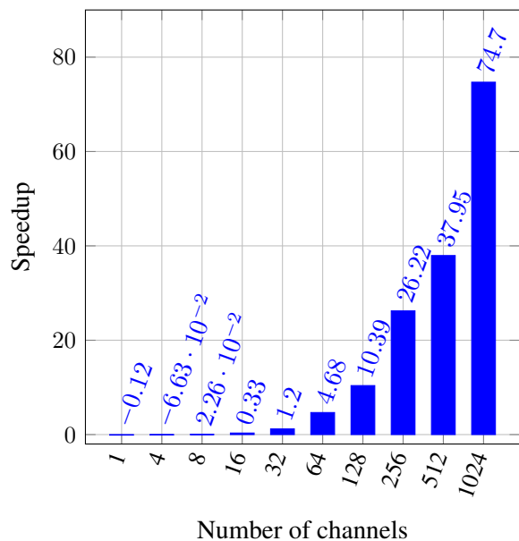
Figure 9: Average DPEPT speedup of the performance over the PT for the benchmark (Fig. 8).
