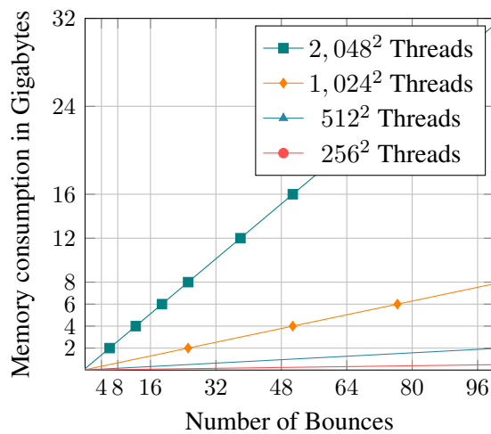
Figure 7: Memory consumption of the DPEPT implementation for different thread pool sizes.
