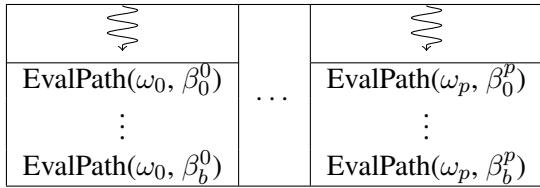
Figure 5: Path parallelization pattern of a work-group (one path per work-item) for the paths evaluation. \omega is a work-item (thread of the work-group). EvalPath( \omega_p, \beta_b^p ) is the evaluation of the path sample p for its wavelength sample batch b (Algorithm 1).
