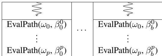
Figure 6: Spectral parallelization pattern of a work-group (wavelength samples batches of different paths per work-item) for the paths evaluation. \omega is a work-item (thread of the work-group). EvalPath(\omega_p, \beta_b^p) is the evaluation of the path sample p for its wavelength sample batch b (Algorithm 1).
