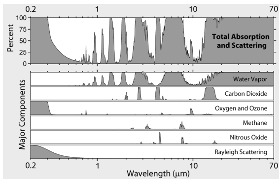
Figure 2: The absorption spectrum of the atmosphere [Roh07] is very spiky.
