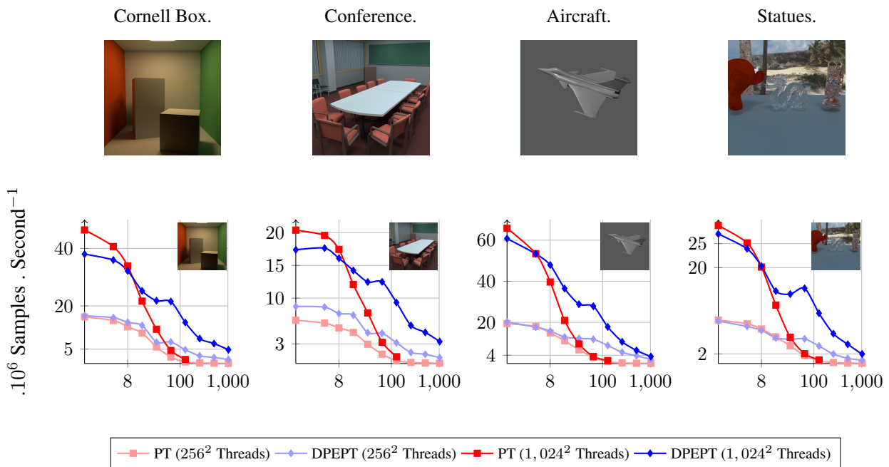
Figure 8: Benchmark with an AMD Fury X (VRAM: 4GB). The scaling of the x-axis is a logarithm base 2.
