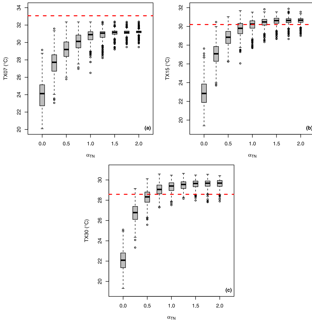
Fig. 11. Boxplots of simulated temperatures for the hottest 7 and 15 days periods starting on June 26, and the 30-day period starting on June 21, as a function of the parameter \alpha_{TN} , with \alpha_{cal} = 4 . The red dashed line is the average TX between June 21 and July 21, 2021.
