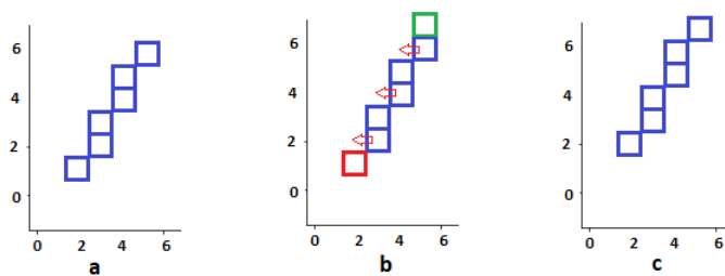
Fig. 3. Soft translation of a vertical segment
