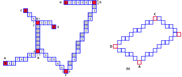
Fig. 4. (a) A DSS tree. The numbers represent the atomic movement order. The red discrete points are the vertices (that have multiple ordre movements, number next to the vertex). The discrete points in gray do not move. (b) A cyclic DSS graph that does not terminate with a naive approach
