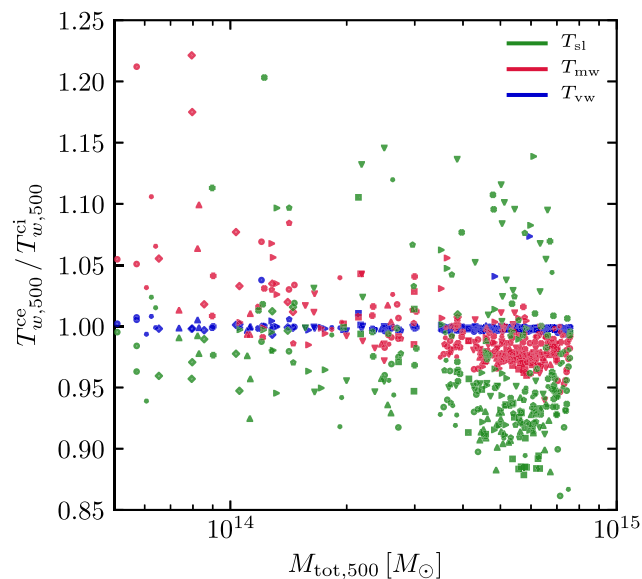
Figure C2. Ratio of the core-excluded to the core-included temperature versus mass for all haloes (NR, MW, VW, and MC combined) with z \leq 1.5 . We show the difference induced by the core exclusion on different temperature estimates: T_{\text{vw}} (blue) and T_{\text{mw}} (red) are a weighted average using respectively the cell volume and the cell density while T_{\text{sl}} (green) uses the cell emissivity and the Mazzotta et al. (2004) weights of hot ( E \geq 0.5 keV) gas cells only.
