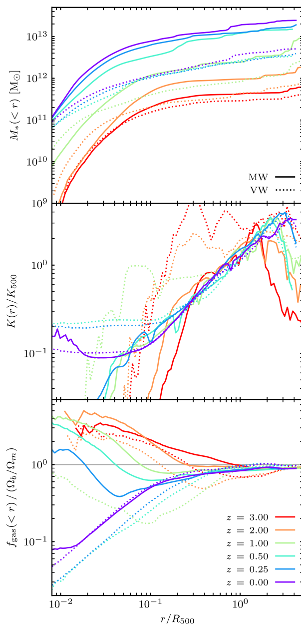
Figure 4. Total enclosed stellar mass (top), ICM entropy (middle), and enclosed gas fraction (bottom) radial profiles. Radii have been normalized to R_{500} corresponding to the radius enclosing 500 times the critical density at the indicated redshift (we have R_{\text{vir}} \sim 1.7 - 2R_{500} ). Solid and dotted lines show the radial profiles of the MW and VW simulations, respectively, and line colour indicates the redshift at which the radial profile is computed. The entropy profiles has been rescaled by the self-similar value K_{500} of Nagai, Kravtsov & Vikhlinin (2007) to compare profiles at different redshifts more easily. The universal baryon fraction is shown in the bottom panel by the horizontal grey line. We see the greater effect of the AGN with a volume weighted energy deposition in quenching star formation at all radii. The entropy profiles indicate that the VW AGN is more efficient in heating the ICM up to large radii at z > 1 . It also allows an earlier transition to a NCC cluster by z = 0.5 , while the MW simulation still shows in the core low entropy and high f_{\text{gas}} values.
