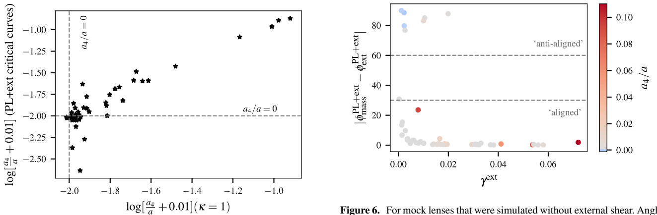
Figure 6. For mock lenses that were simulated without external shear. Angle between the best-fitting values of external shear and the major axis of the lens mass distribution, |\phi_{\text{mass}}^{\text{PL+ext}} - \phi_{\text{ext}}^{\text{PL+ext}}| in degrees, as a function of the amplitude of the best-fit external shear, \gamma^{\text{ext}} . Points are coloured by the magnitude of the inferred critical curves deviation from elliptical symmetry a_4/a , values of a_4/a < 0 correspond to boxy critical curves and a_4/a > 0 to discy ones. Values are orders of magnitude different, with the lowest values going down to 0.001.
