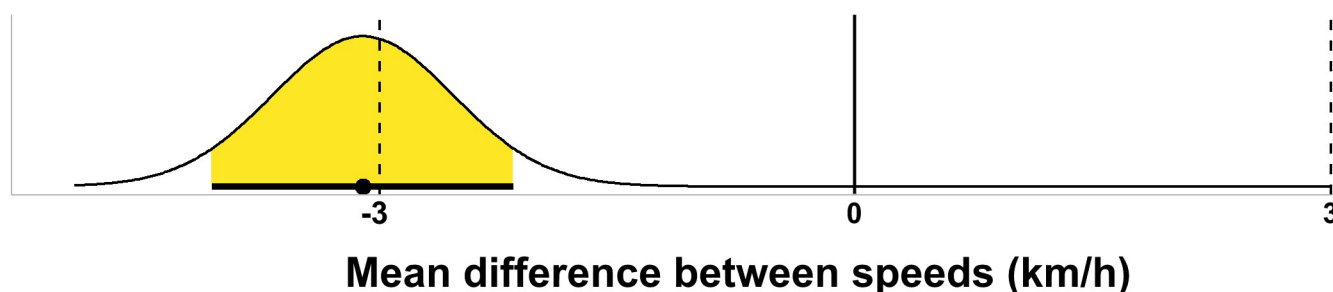
Fig 1. Consonance density plot of the difference between the two speeds, combining all experimental conditions. Note. The yellow area indicates the 90% confidence intervals from the two one-sided tests procedure. The dashed vertical black lines indicate the equivalence bounds (in raw scores) and the vertical black line indicates the nil null hypothesis.
