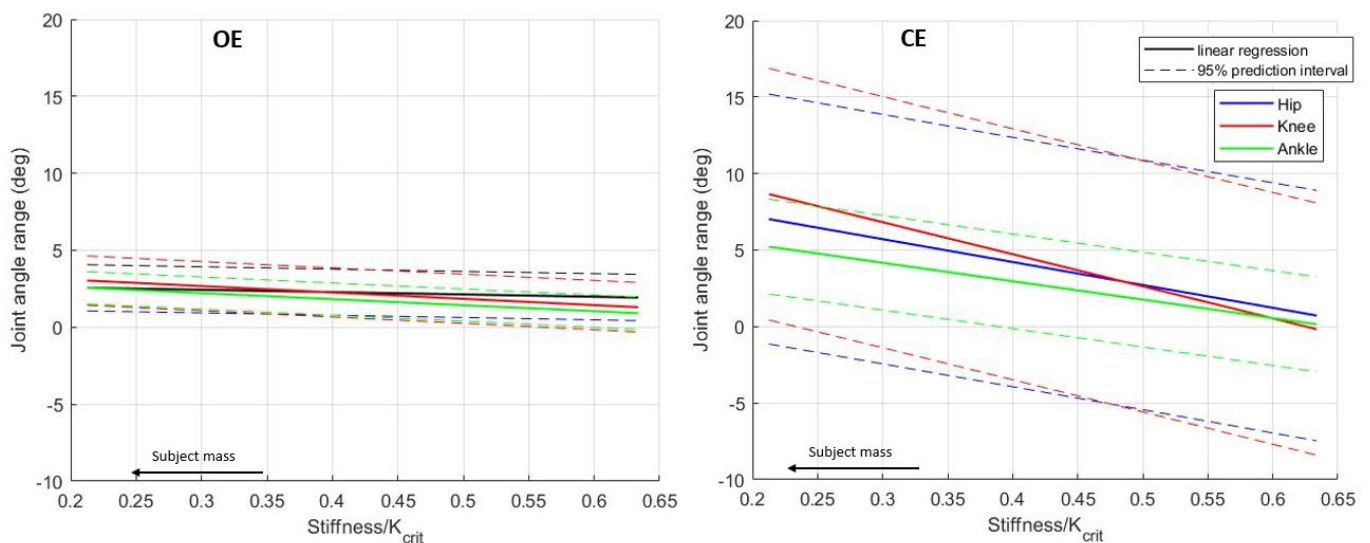
Figure 6. Linear regression of the joint angles ROM as a function of the normalized ankle stiffness in the OE (left) and CE (right) situation.
