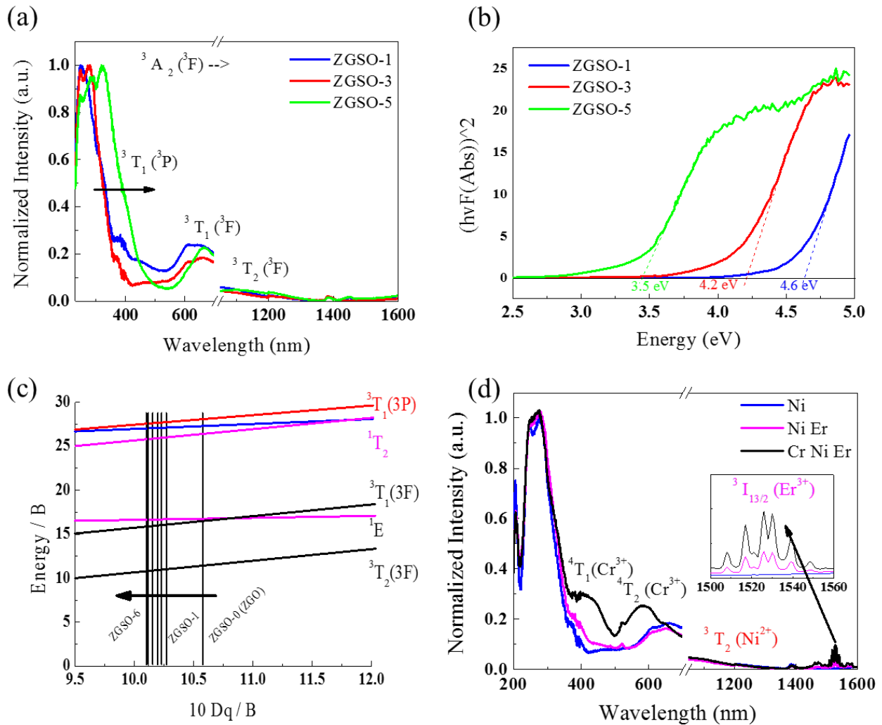
Figure 2. (a) Normalized absorption spectra of samples Ni 2+ -doped ZGSO-1 ( \text{Zn}_{1.1}\text{Ga}_{1.79}\text{Ni}_{0.01}\text{Sn}_{0.1}\text{O}_{3.995} ), ZGSO-3 ( \text{Zn}_{1.3}\text{Ga}_{1.39}\text{Ni}_{0.01}\text{Sn}_{0.3}\text{O}_{3.995} ), and ZGSO-5 ( \text{Zn}_{1.5}\text{Ga}_{0.09}\text{Ni}_{0.01}\text{Sn}_{0.5}\text{O}_{3.995} ). (b) Bandgap calculation of samples Ni 2+ -doped ZGSO-1, ZGSO-3, and ZGSO-5. (c) Part of the Tanabe–Sugano diagram of Ni 2+ with d 8 electron configuration in the complex spinel samples of ZGSO-0~ZGSO-6 with different Sn concentrations (see Table S3). (d) Transition-metal (Ni 2+ and/or Cr 3+ ) and rare-earth (Er 3+ ) doped ZGSO-3. The illustration is a partial enlargement of Er 3+ absorption.
