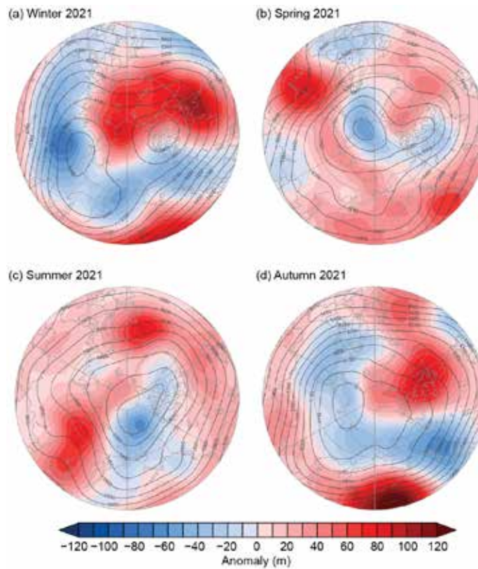
Fig. 5.3. Seasonal atmospheric circulation patterns in 2021 for (a) winter, (b) spring, (c) summer, and (d) autumn. The contours (shading) represent 500-hPa geopotential height values (anomalies relative to the 1991–2020 seasonal means, m). Upper-level winds tend to circulate clockwise around higher geopotential height values. (Source: ERA5 reanalysis geopotential height data are obtained from the Copernicus Climate Change Service.)
