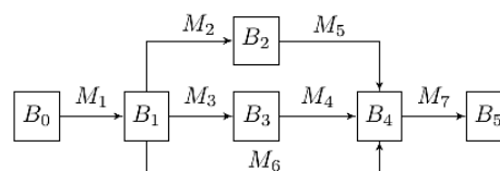
Fig. 1. Example of a line with a series-parallel network
