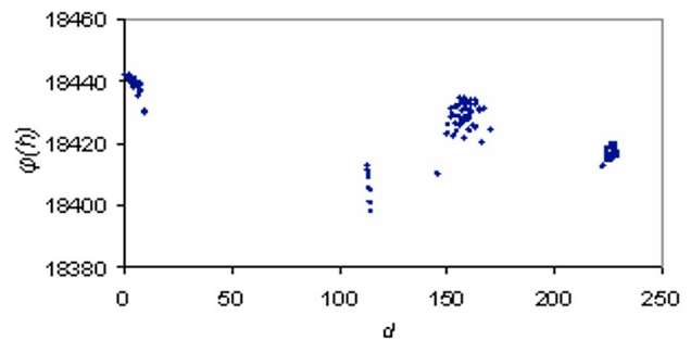
Fig. 8. Final population of the GA with local optimization heuristic on instance as.4 (note that here the scale of both axes is different from that in Figures 4 and 7)
