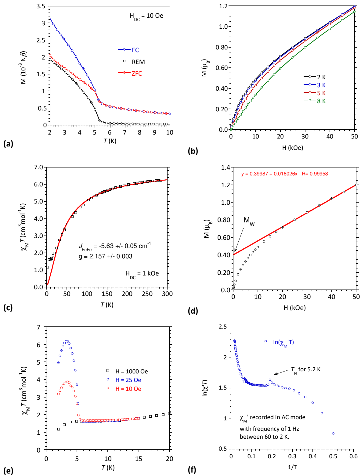
Figure S5. Magnetic behaviors for [\text{FeL}^{\text{N5R,R}}\{\text{FeCl}_4\}] , 2R : (a) Field-cooled (FC), zero-field cooled (ZFC), and remanent magnetization recorded with H_{\text{DC}} = 10 Oe; (b) M versus H behaviors between 2 and 8 K; (c) \chi_M T versus T obtained with H = 1 kOe: experimental ( \square ) and calculated ( - ), fit between 300 and 17 K, the part down to 2 K is an extrapolation); (d) \chi_M T versus T between 25 and 2 K obtained for H = 1000 Oe, 25 Oe, and 10 Oe; (f) \ln(\chi_M T) versus 1/T recorded for \nu = 1 Hz.
