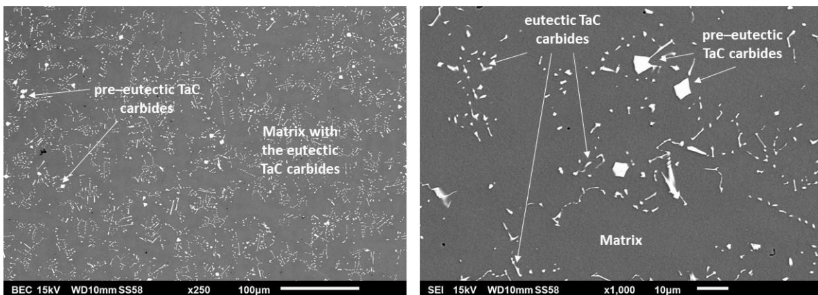
Figure 3: Low (left) and high (right) magnification SEM/BSE pictures illustrating the as-cast microstructure of the “TAhea” alloy.
