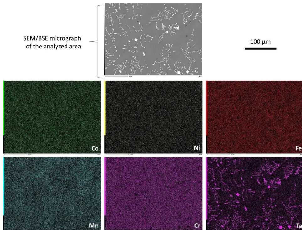
Figure 5: EDS elemental repartition maps in the “TAhea” alloy’s microstructure.
