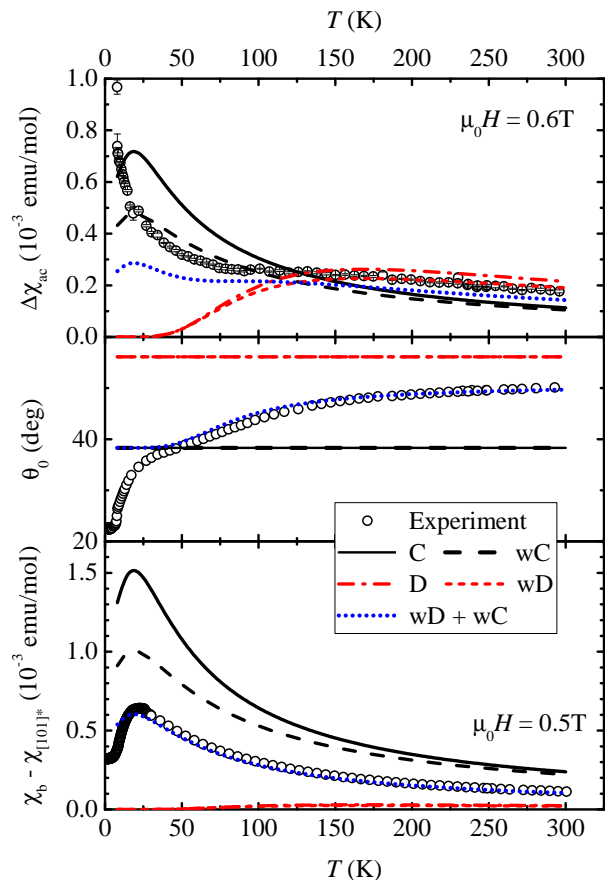
Figure 5. Temperature dependence of susceptibility anisotropy measured in the ac plane and plane spanned by (b, [101]^*) axes (top and bottom panel), in \mu_0 H = 0.6 T and 0.5 T, respectively. Middle panel: Temperature dependence of the torque phase \theta_0 which corresponds to the direction of magnetic eigenaxis in the ac plane. The results for C, wC, D, wD and wC+wD models are shown by black solid, black dashed, red dashed, red dotted and blue dotted lines, respectively.
