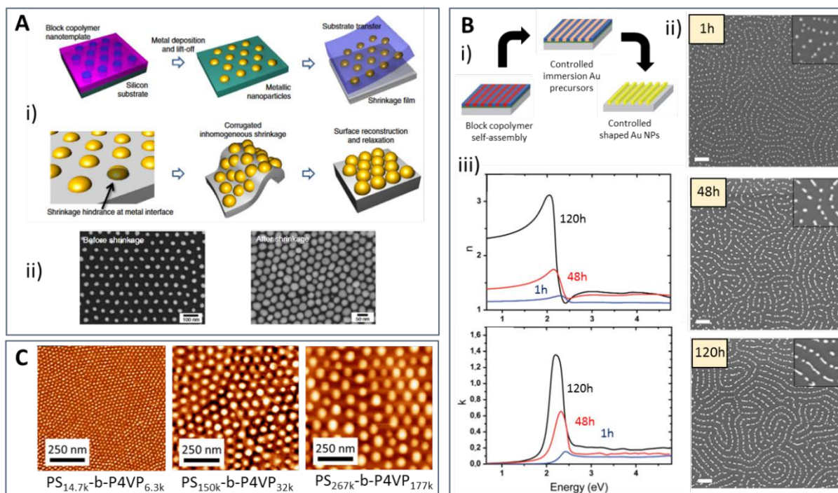
Figure 11. A) i) Schematic for metal NP metasurface preparation by BCP self-assembly ii) SEM images of hexagonal gold NP arrays as-prepared from BCP self-assembly (left) and after complete pattern shrinkage (right). Reproduced with permission [72] . Copyright 2016, Springer Nature. B) i) schematic illustration of the fabrication of the gold decorated surfaces derived from nanostructured BCP thin films ii) SEM images of discrete gold nanoparticle arrays formed on a silicon substrate using a PS- b -P2VP BCP template by immersion in aqueous gold precursor solution for different times. iii) Refractive index of the studied nanostructured surfaces. Reproduced with permission [240] . Copyright 2019, Royal Society of Chemistry. C) AFM topographical images of the three sizes gold NP hexagonal arrays obtained using three different molecular weight BCP as template. Reproduced with permission [243] . Copyright 2020, AIP Publishing.
