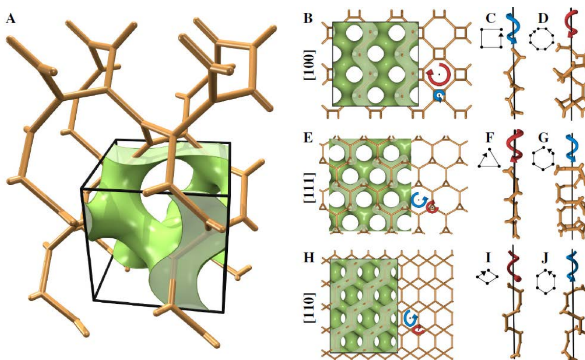
Figure 8. The single gyroid morphology at 20% volume fill fraction (green) and its underlying srs network (brown). (A) Perspective view of a single cubic unit cell. (B,E,H) Projections onto the fundamental crystallographic directions (smallest Miller indices). Chiral right-handed (red) and left-handed (blue) helical elements of the srs are highlighted with curved arrows. The small
