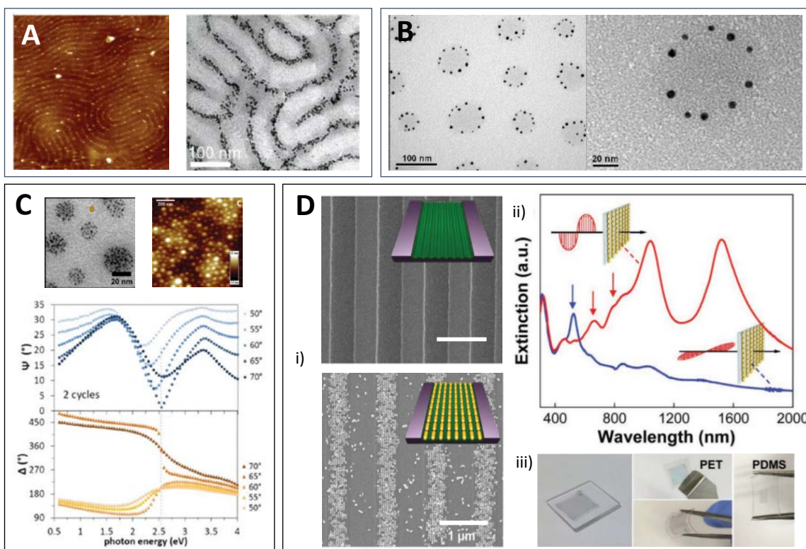
Figure 10. A) AFM (left) and TEM (right) images of PS-b-P2VP/gold nanoparticle hybrid thin films. Particles are located at P2VP domains through the control of their surface chemistry. Reproduced with permission [163] . Copyright 2008, Wiley-VCH. B) TEM of the gold nanoparticles forming rings at the interface between the PS domains and the PMMA matrix. Reproduced with permission [167] . Copyright 2013, American Chemical Society. C) AFM and TEM images of the PVP domain containing gold nanoparticles formed by sonication (top) and ellipsometric angles as a function of photon energy for different angles of incidence for the film obtained. Reproduced with permission [164] . Copyright 2018, Royal Society of Chemistry. D) i) SEM image of linearly aligned grooves of plasma-treated PS-b-PMMA thin film on the lithographic pattern (top) and gold NRs deposited on the aligned grooves (bottom). ii) Polarization-dependent extinction spectra of aligned gold NRs on quartz substrate. iii) Photos of transferred gold NRs to various substrates. Reproduced with permission [253] . Copyright 2019, Wiley-VCH.
