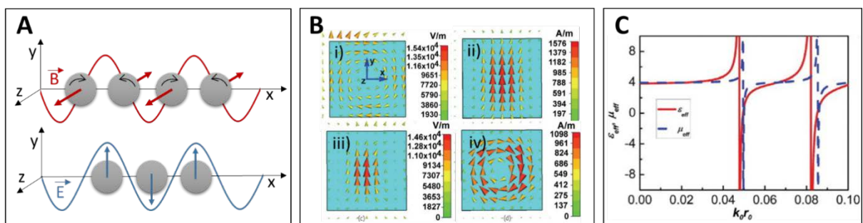
Figure 2 The magnetic dipole (top) and electric dipole (bottom) oscillating with the incident electric field of light. (B) Electric (left, z = 0 plane) and magnetic (right, y = 0 plane) field distribution in a dielectric cube near the first Mie resonance (top) and near the second Mie resonance (bottom). Reproduced with permission [87] . Copyright 2008, American Physical
