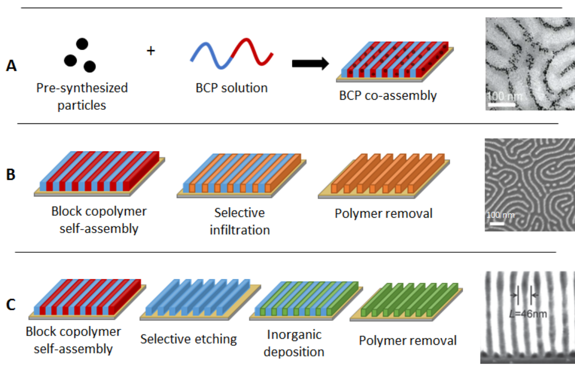
Figure 7. Schematics of the different strategies followed to design optical metamaterials architectures using BCP films as a template: A) BCP co-assembly (Reproduced with permission [169] ; Copyright 2008 Wiley-VCH) B) selective infiltration, (Reproduced with permission [68] , Copyright 2019 Royal Society of Chemistry) and C) Inorganic deposition, (Reproduced with permission [169] , Copyright 2014 Wiley-VCH).
