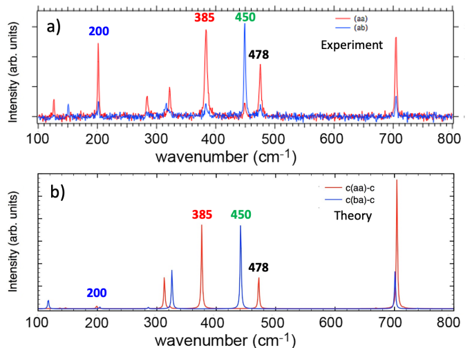
FIG. 3. Comparison of the (a) experimental spectra of \text{SrCu}_2(\text{BO}_3)_2 measured at 7 K and (b) theoretical Raman spectra for two polarizations. The energy of the theoretical spectra has been stretched by 7%. The four intense experimental phonon modes involving Cu-O bonds whose schematic representation are shown in Fig. 5 are labeled in the spectra (see text).
