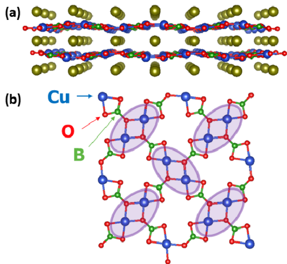
FIG. 1. Atomic structure of \text{SrCu}_2(\text{BO}_3)_2 (a) along the [100] direction and (b) along the [001] direction. Sr atoms are in yellow, O in red, B in green, and Cu in blue. The buckling of the [\text{CuBO}_3]^- layers along the [001] direction is visible in (a). The orthogonal Cu dimers have been highlighted in magenta in (b). Atomic structures were drawn with VESTA [17].
