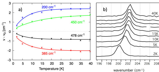
FIG. 4. (a) Evolution of the energy of four Raman modes of \text{SrCu}_2(\text{BO}_3)_2 at B=0 with temperature and (b) waterfall plot showing the evolution of the energy of the peak at 200\text{ cm}^{-1} with temperature. In (a), the lines are exponential fits to the experimental points that extrapolate to zero at zero temperature. They must be considered as guides to the eye.
