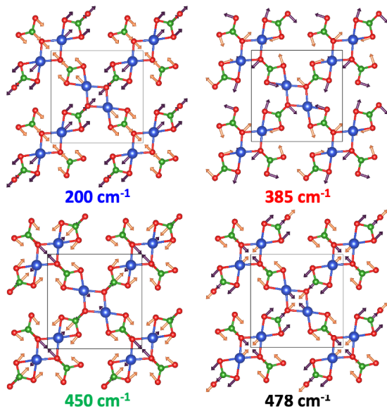
FIG. 5. Schematic representation of the phonon modes of \text{SrCu}_2(\text{BO}_3)_2 with strongest temperature and magnetic field dependence. The lengths of the arrows are proportional to the atomic displacements. Phonon mode visualizations were drawn with VESTA [17]. Displacement diagrams labeled 200\text{ cm}^{-1} and 450\text{ cm}^{-1} show Cu and O atom motion consistent with the pantograph modes, while 385\text{ cm}^{-1} and 478\text{ cm}^{-1} are non-pantograph .
