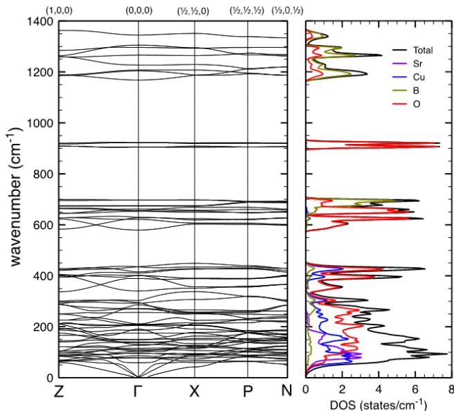
FIG. 2. Phonon band structure and projected density of states of \text{SrCu}_2(\text{BO}_3)_2 .
