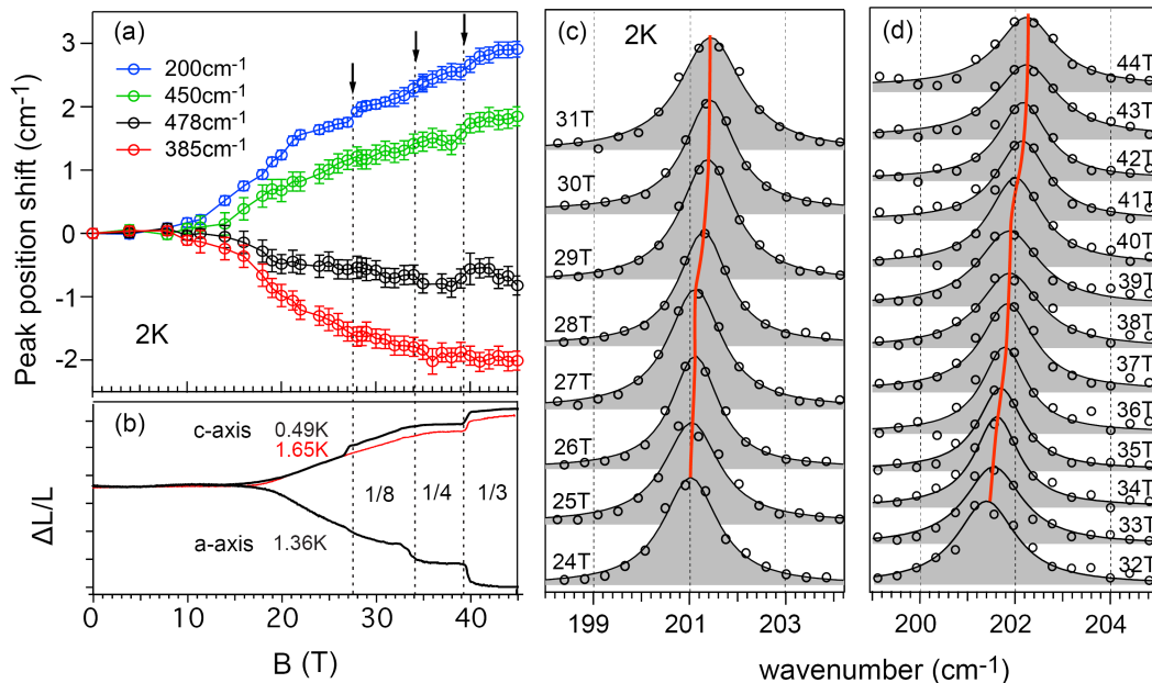
FIG. 6. (a) Evolution of the energy of four Raman modes of \text{SrCu}_2(\text{BO}_3)_2 with applied magnetic fields up to 45 T. The arrows point to the anomalies detected in 200 \text{ cm}^{-1} mode coinciding with M/M_s = 1/8, 1/4, and 1/3 phases. The energy of the modes was obtained from Lorentzian fit of the average spectrum over multiple spectra obtained at each magnetic field step. The error bars were obtained from the data deviation at each spectrum in the group. (b) Magnetostriction of \text{SrCu}_2(\text{BO}_3)_2 along a and c crystallographic axes measured at magnetic fields up to 45 T. Adapted from Ref.[10]. (c) and (d) Evolution of the 200 \text{ cm}^{-1} pantograph phonon mode with respect to increasing magnetic fields in the range 24 - 44 T. The data points are shown as open circles and the solid lines are the Lorentzian fit of the data.
