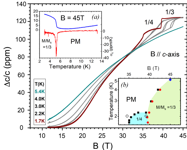
FIG. 7. Main panel: c -axis magnetostriction measured to 45T at different temperatures between 1.7K and 5.4K. Inset (a): Thermal expansion \Delta c/c (left y -axis) and coefficient of thermal expansion \alpha (right y -axis) vs temperature measured at constant magnetic field B = 45 T, showing a sharp phase transition at 5.2K. Inset (b): B, T phase diagram from magnetostriction \Delta c/c vs field (black and red symbols), thermal expansion \Delta c/c vs temperature (blue symbol), and magneto-Raman measurements (open circles). Note that only lines above T = 1.5 K are displayed due to the base temperature of our 4He fridge.
